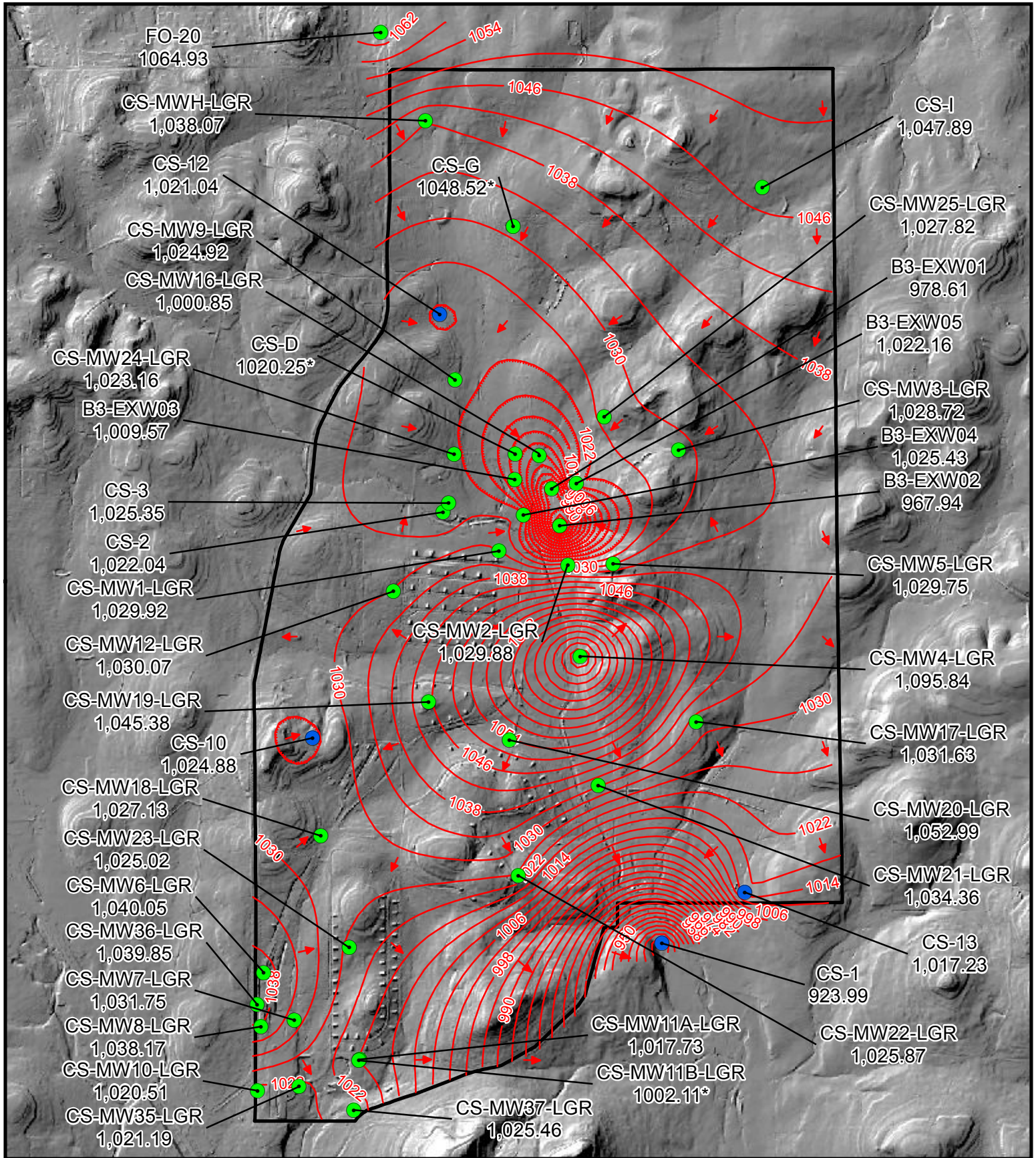
Figure 2.1 June 2020 Potentiometric Surface Map, LGR Wells Camp Stanley Storage Activity PARSONS
