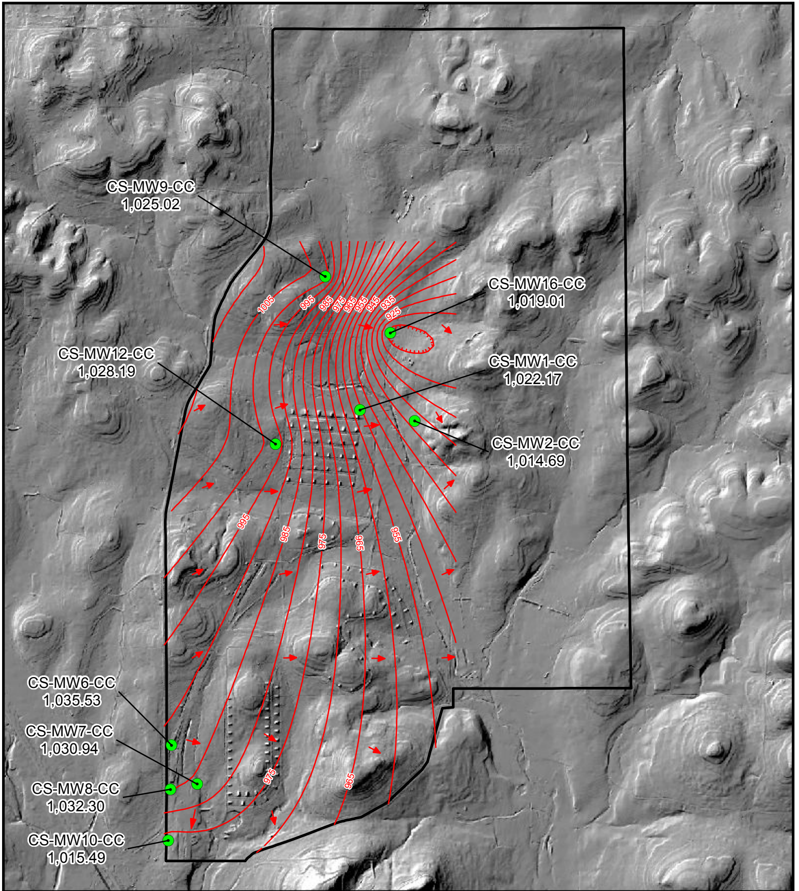
Figure 2.3 June 2020 Potentiometric Surface Map, CC Wells Camp Stanley Storage Activity PARSONS
