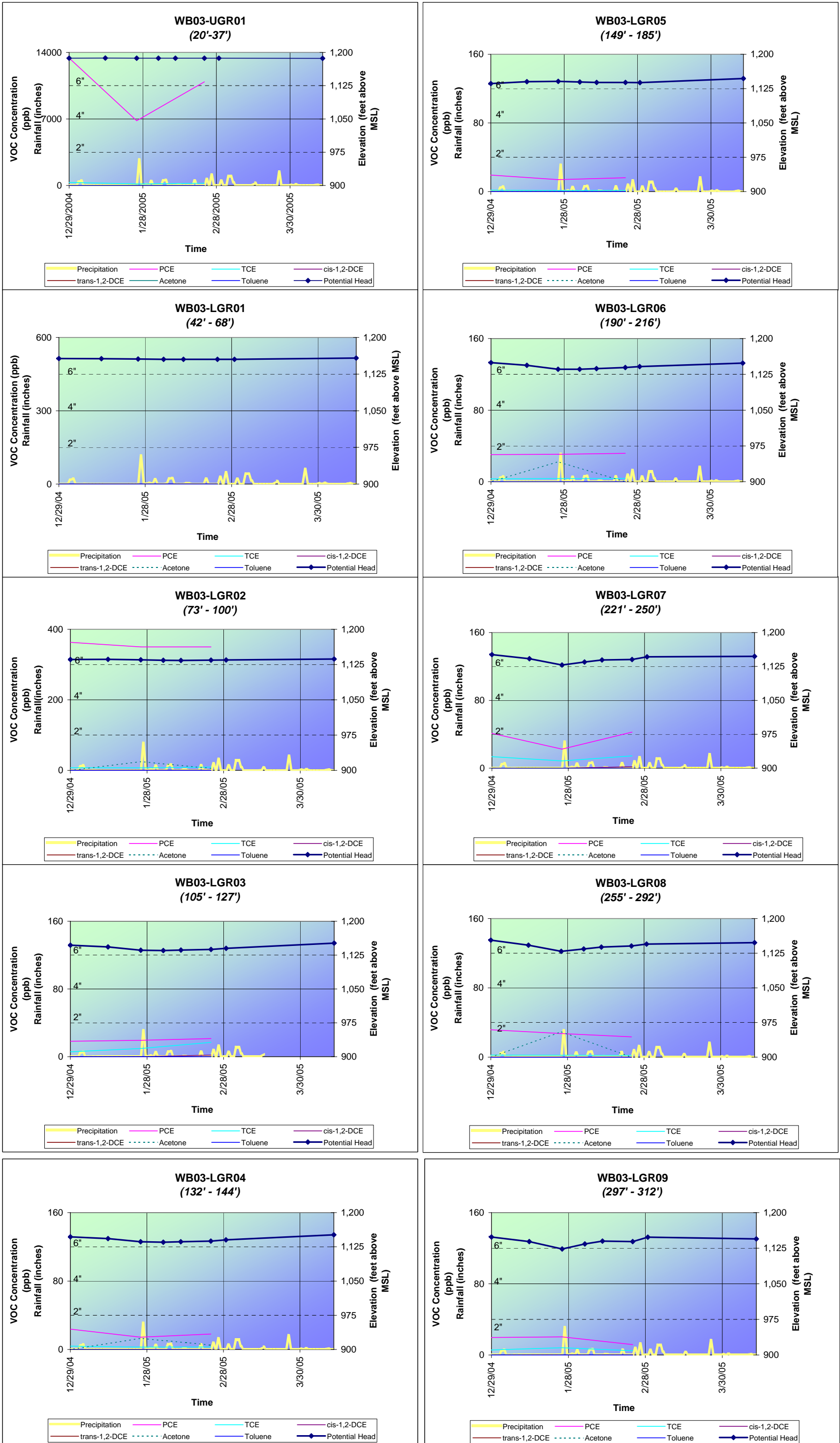
Figure 4-3 CS-WB03 Combined Concentration, Water Level, and Rainfall Data
