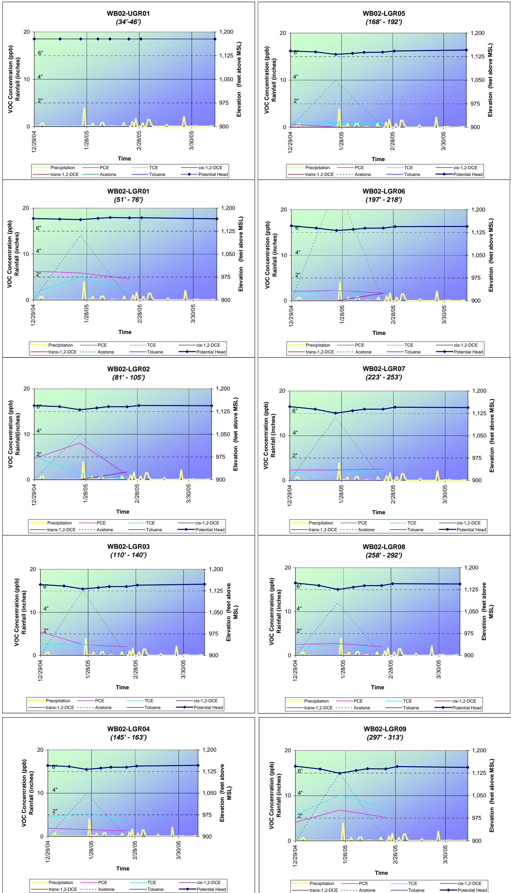
Figure 4-2 CS-WB02 Combined Concentration, Water Level, and Rainfall Data
