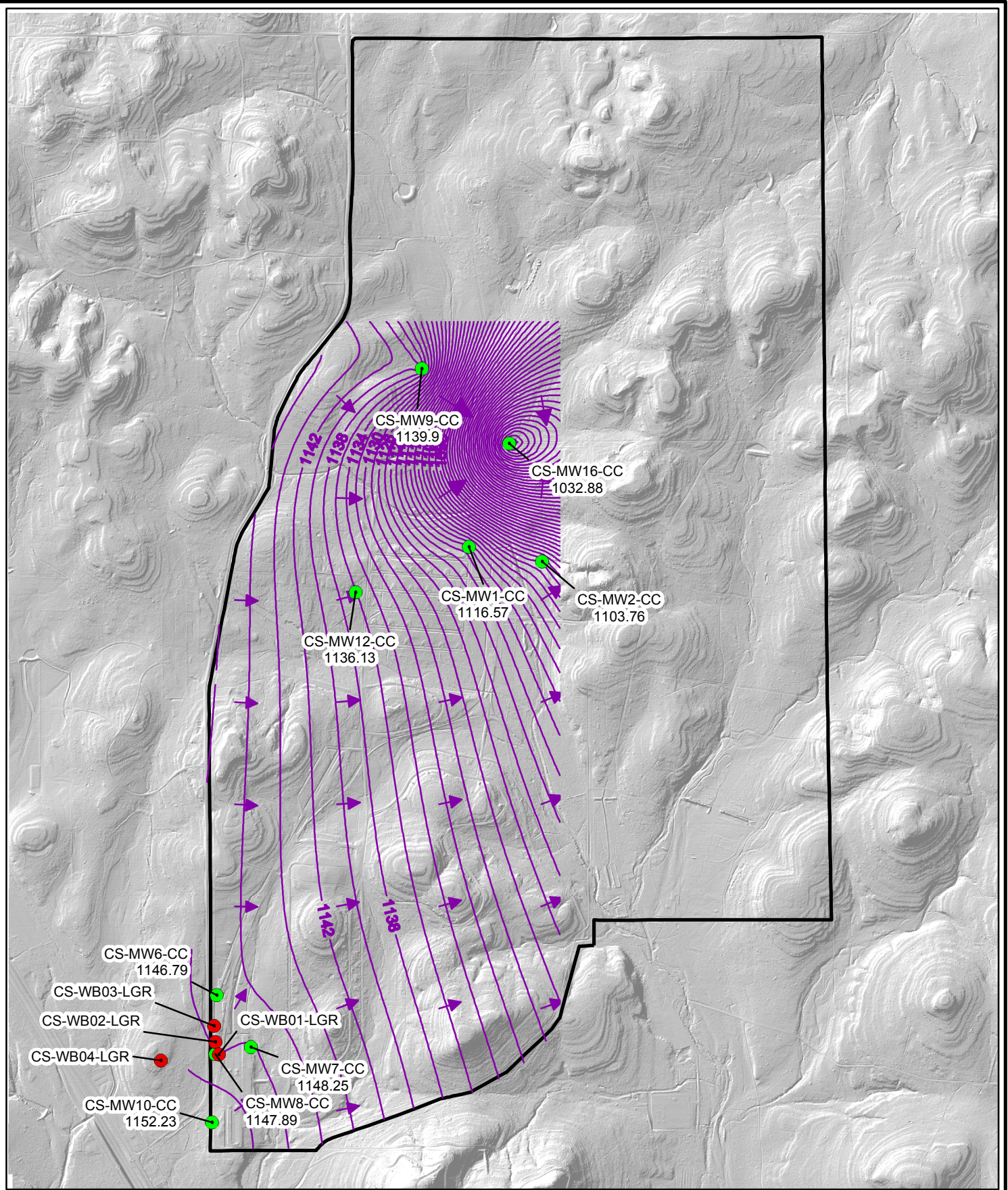
Figure 2-3 March 2005 Potentiometric Surface Map, CC Wells Camp Stanley Storage Activity PARSONS
