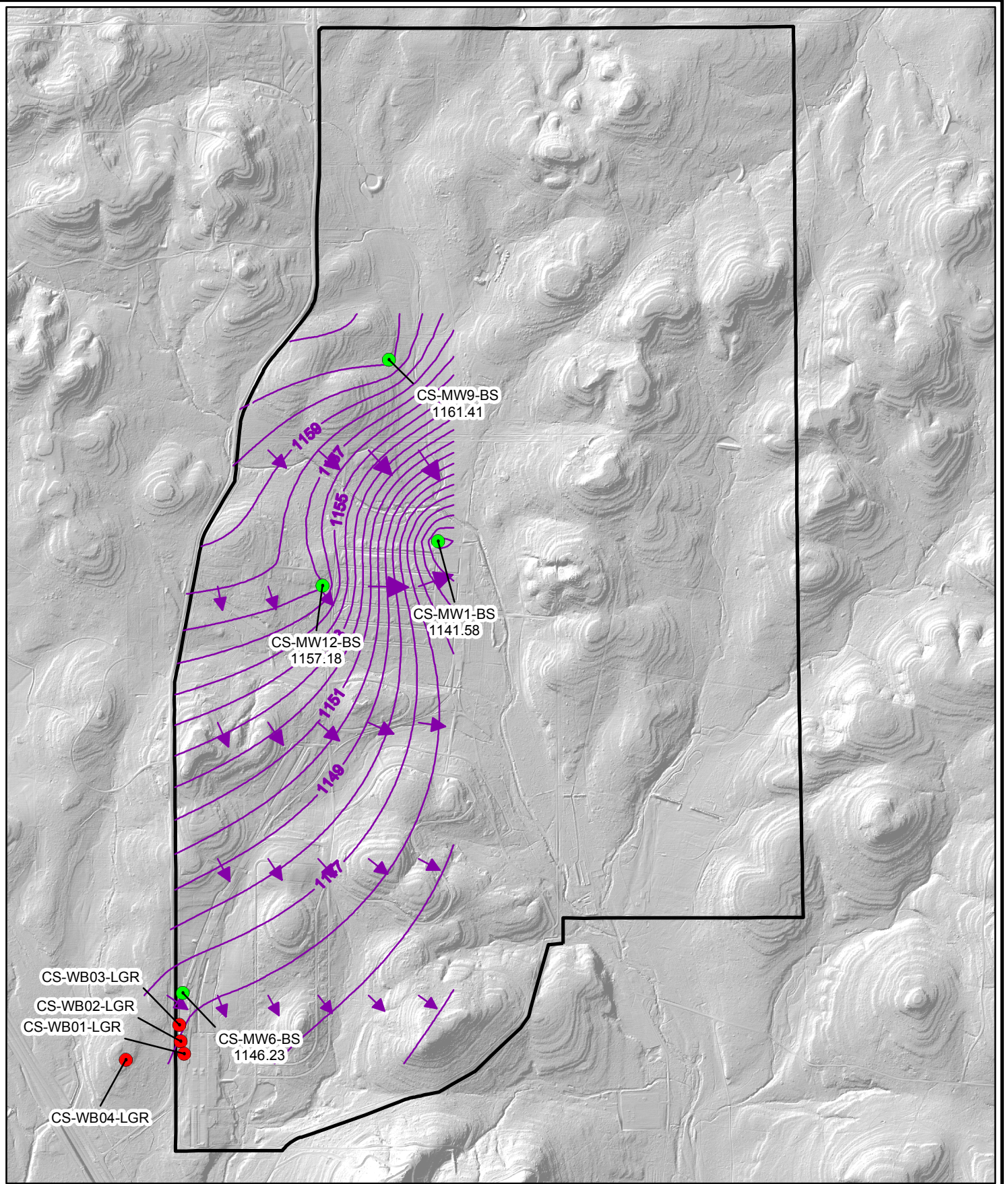
Figure 2-2 March 2005 Potentiometric Surface Map, BS Wells Camp Stanley Storage Activity PARSONS
