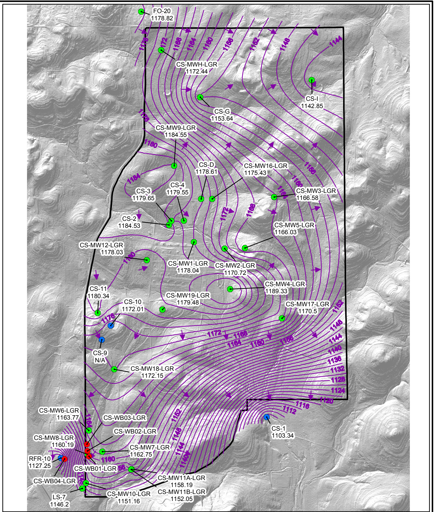
Figure 2-1 March 2005 Potentiometric Surface Map, LGR Wells Camp Stanley Storage Activity PARSONS
