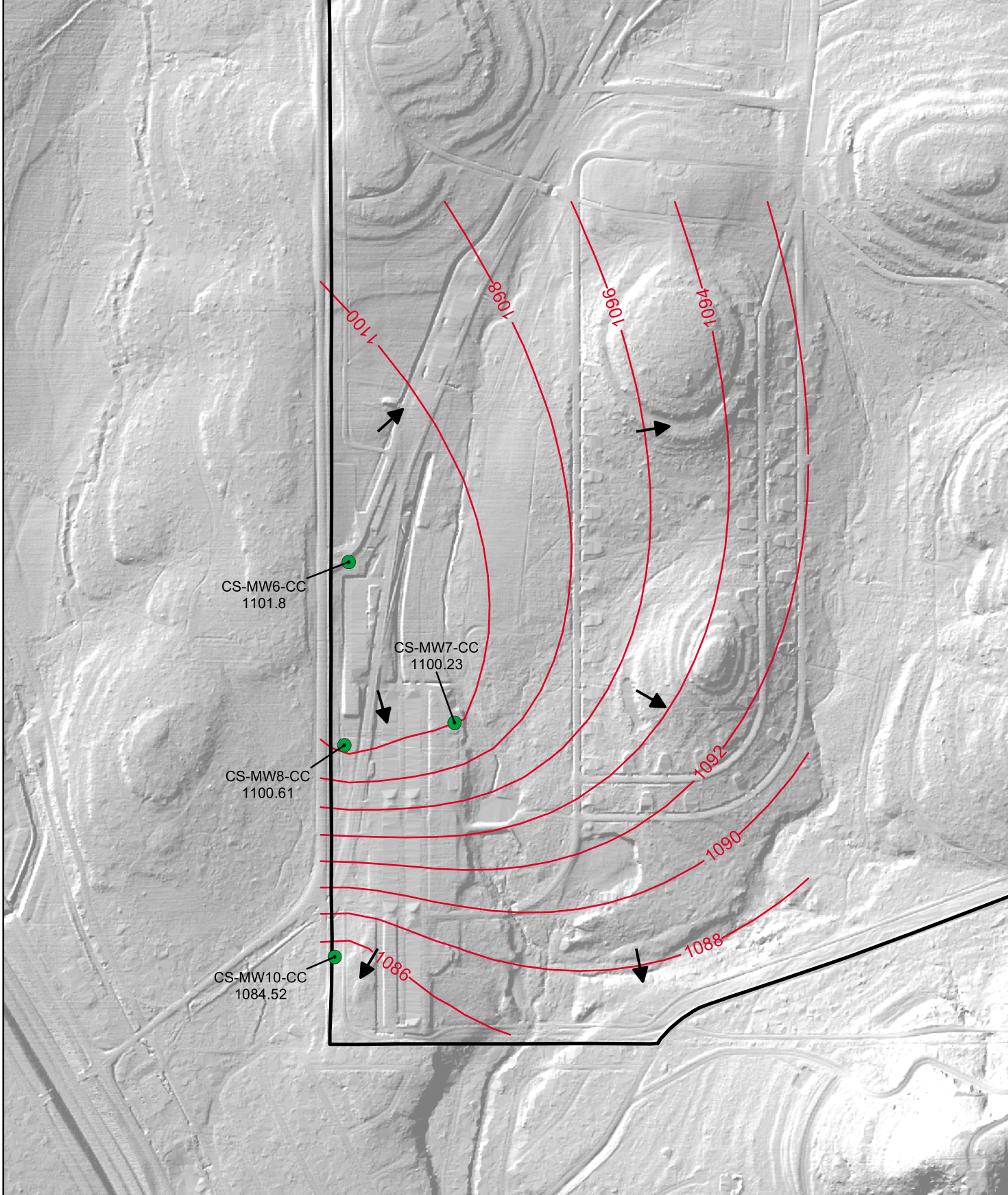
Figure 2-5 September 2004 Potentiometric Surface Map for CC Screened Wells near Building 90 Camp Stanley Storage Activity PARSONS
