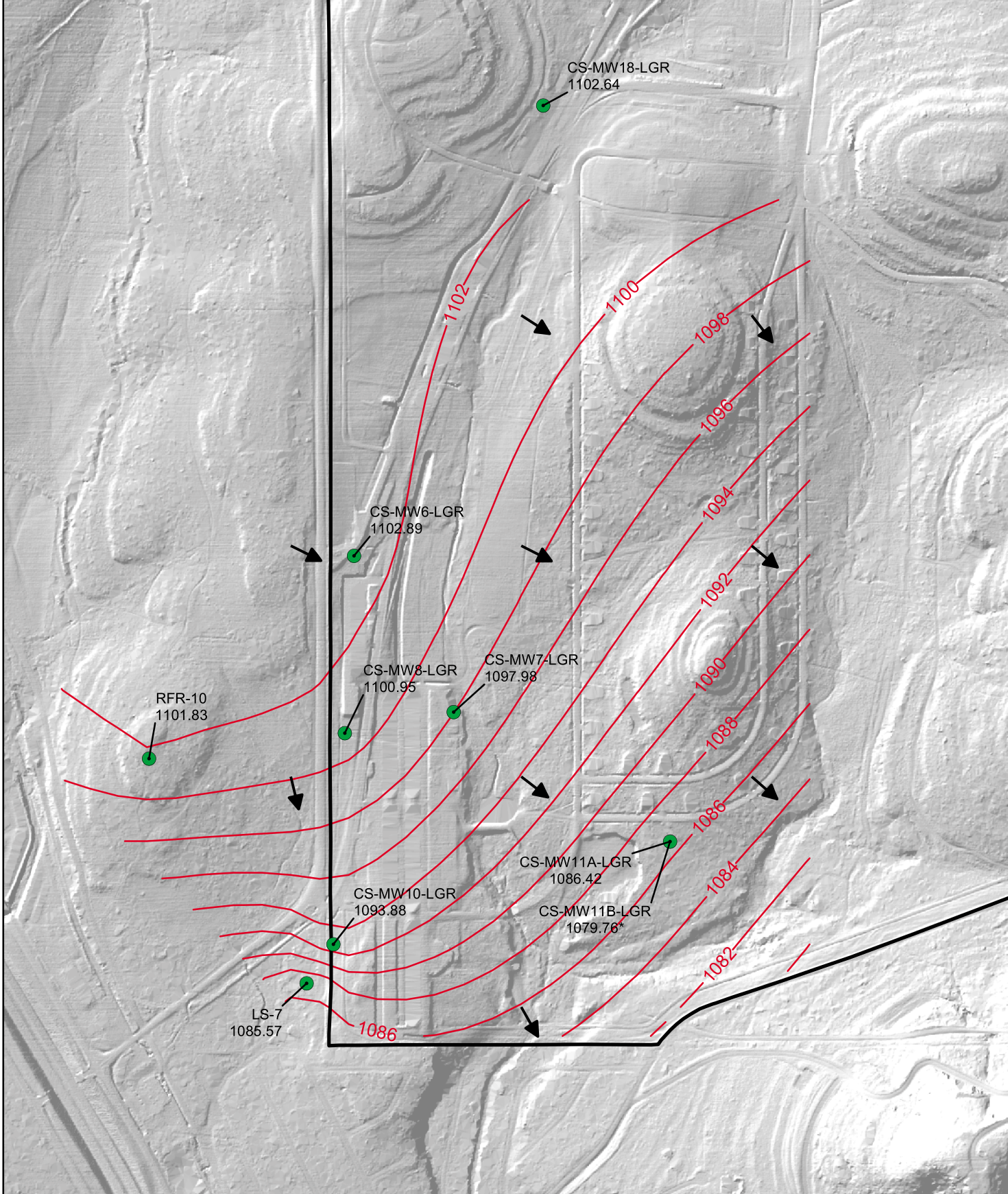
Figure 2-4 September 2004 Potentiometric Surface Map for LGR Screened Wells near Building 90 Camp Stanley Storage Activity PARSONS
