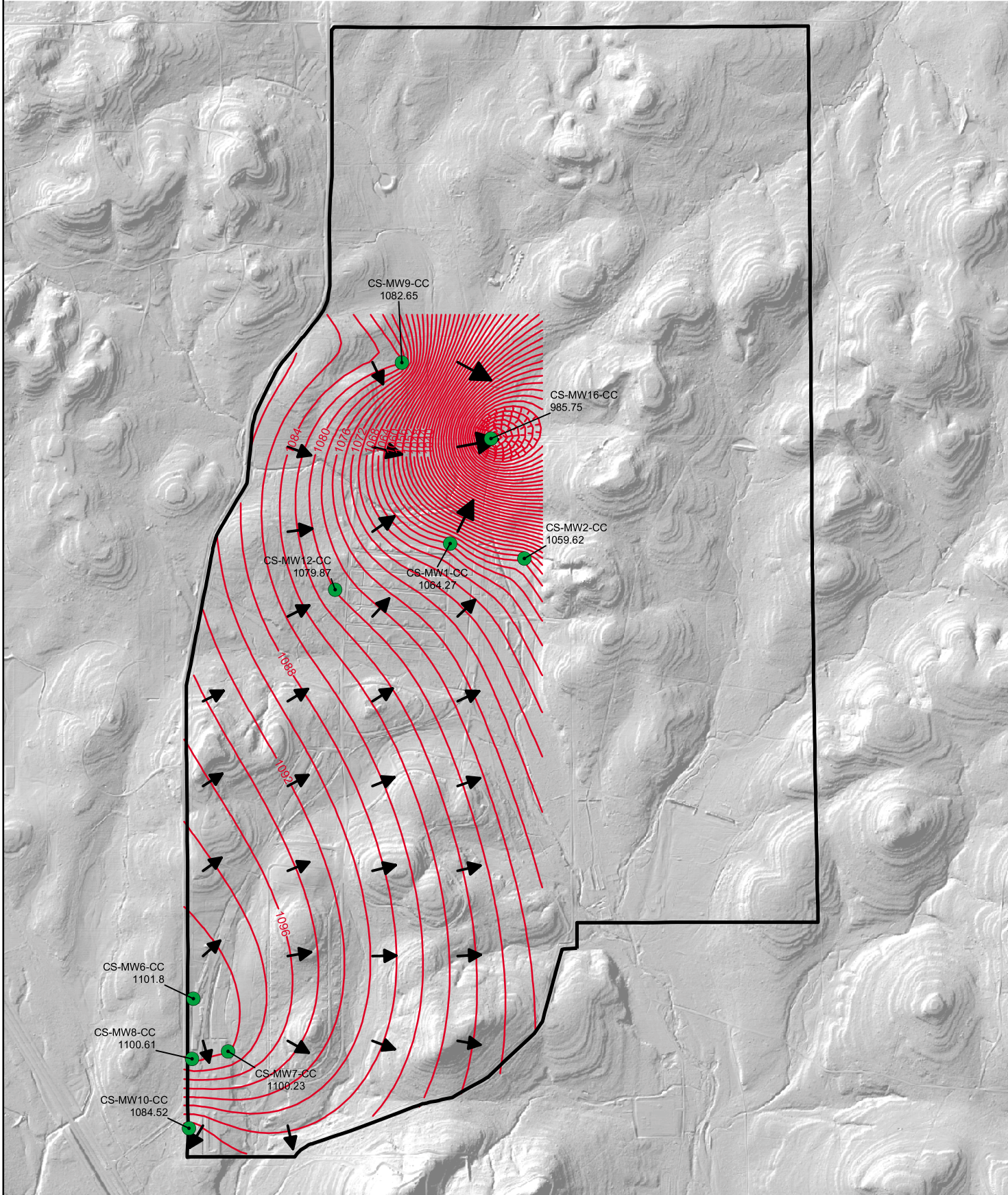
Figure 2-3 September 2004 Potentiometric Surface Map, CC Wells Camp Stanley Storage Activity PARSONS
