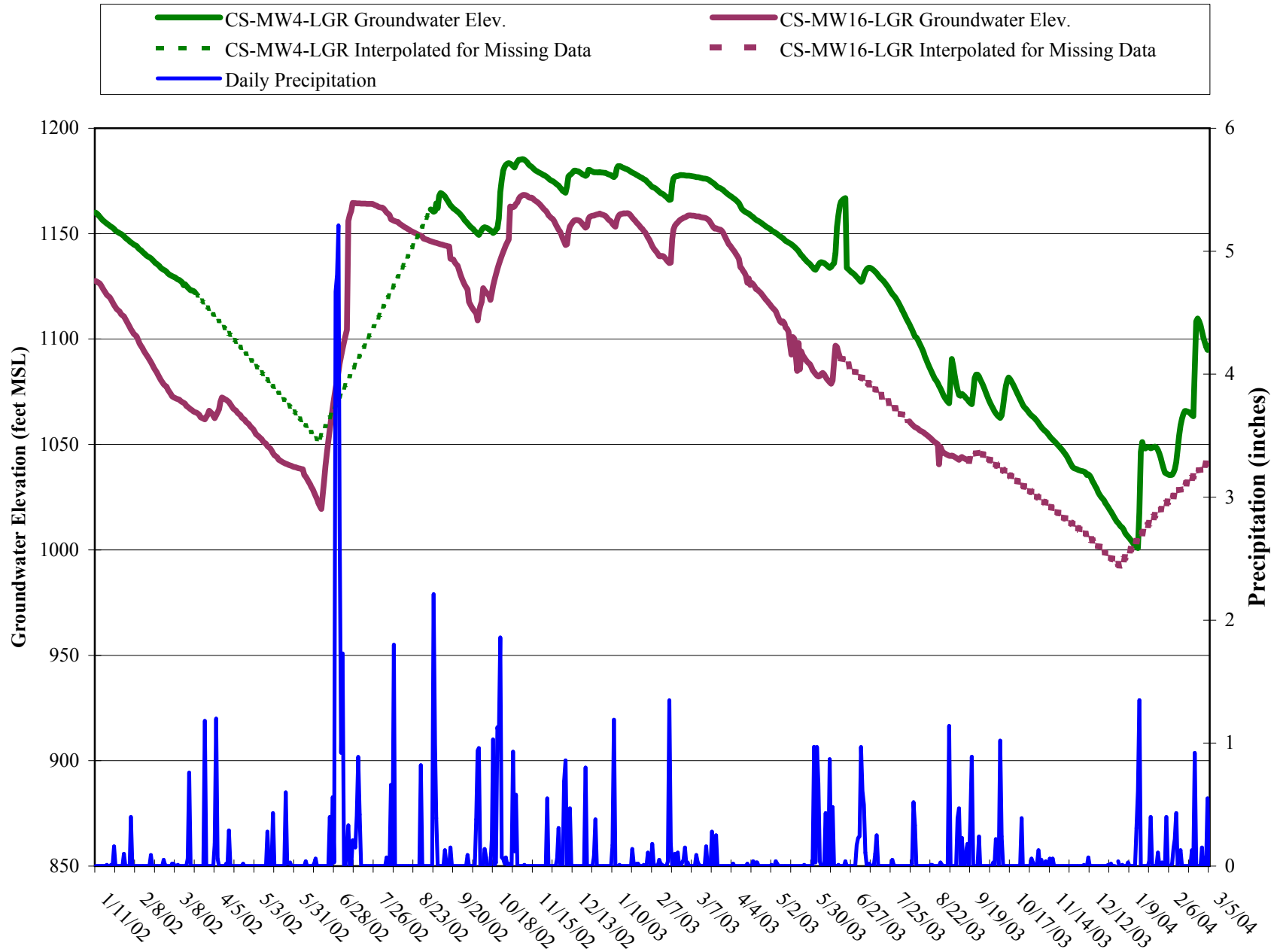
Figure 3-3, Wells CS-MW16-LGR and CS-MW4-LGR Groundwater Elevations and Precipitation Data, through March 2004
