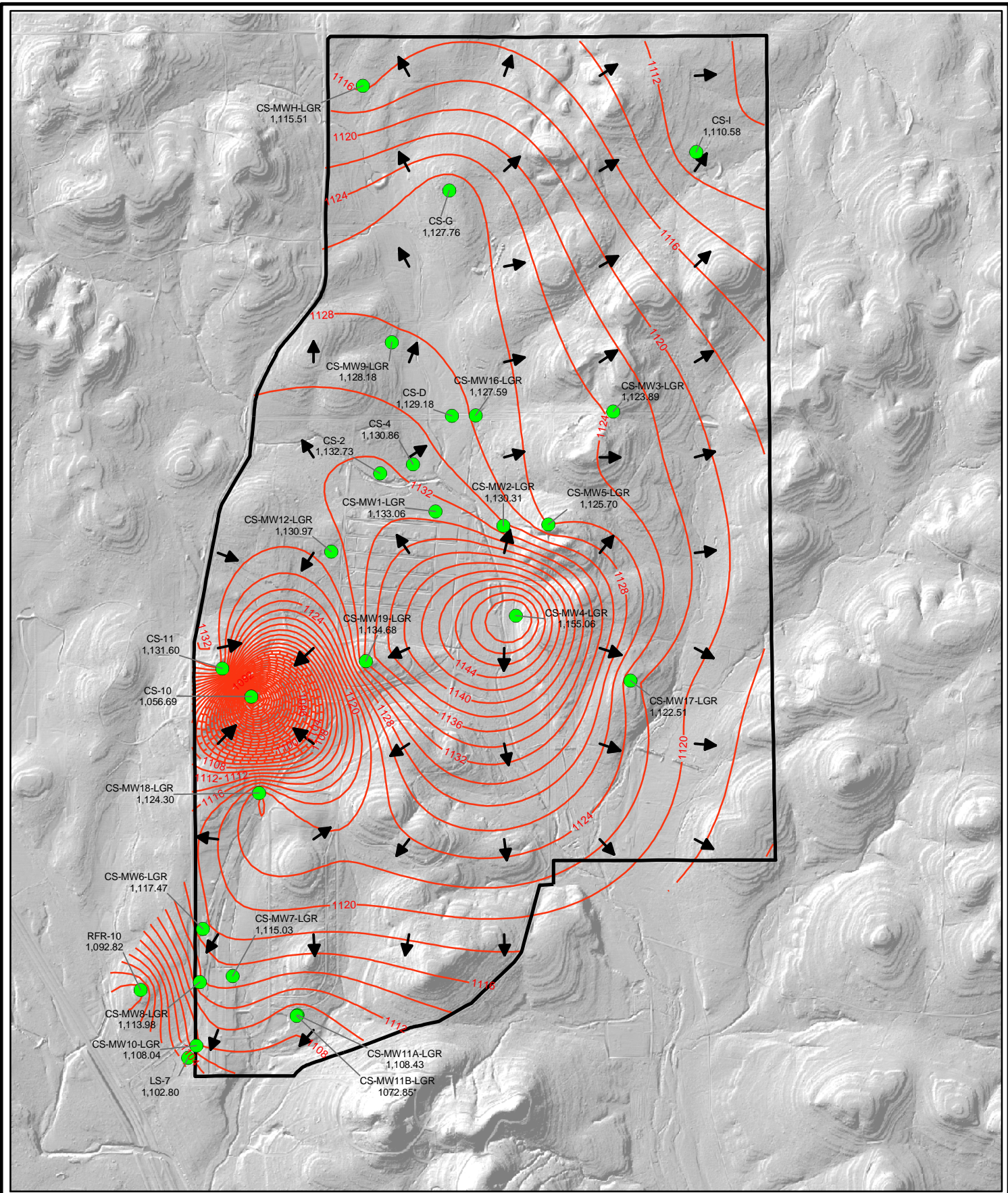
Figure 2-1 June 2004 Potentiometric Surface Map, LGR Wells Camp Stanley Storage Activity PARSONS
