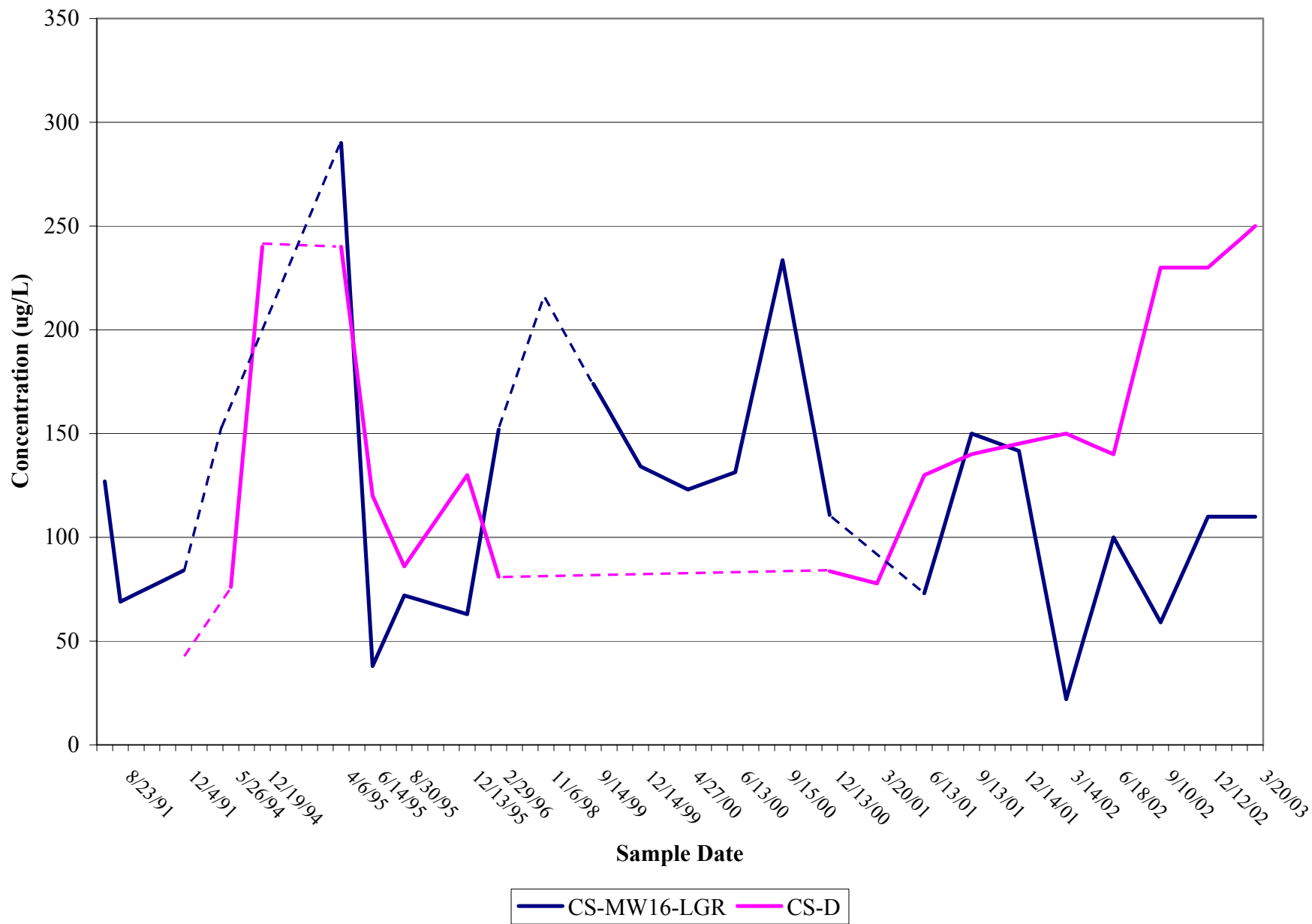
Figure 5-3, Concentrations of cis -1,2-Dichloroethene in Selected Wells MCL = 70 ug/L
