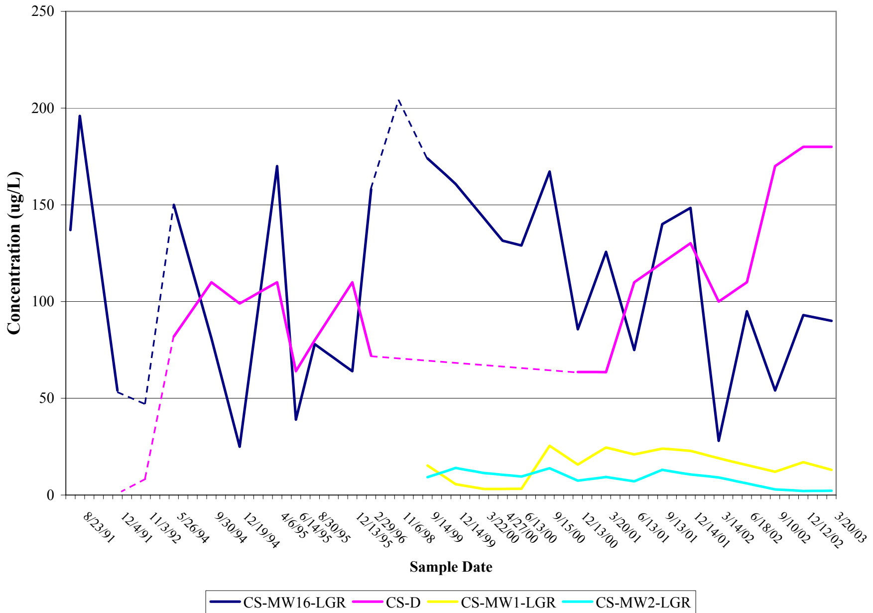
Figure 5-1, Concentrations of Tetrachloroethene in Selected Wells MCL = 5 ug/L
