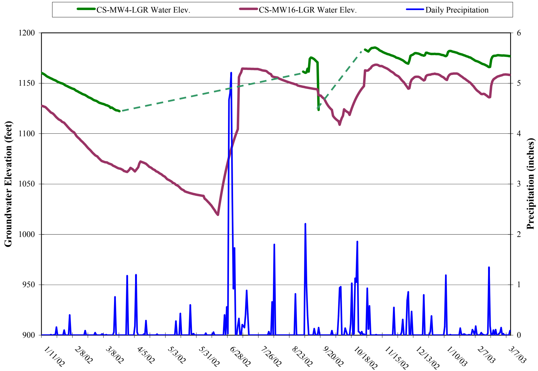
Figure 3-3, Wells CS-MW16-LGR CS-MW4-LGR Groundwater Elevations and Precipitation Data, March 2003
