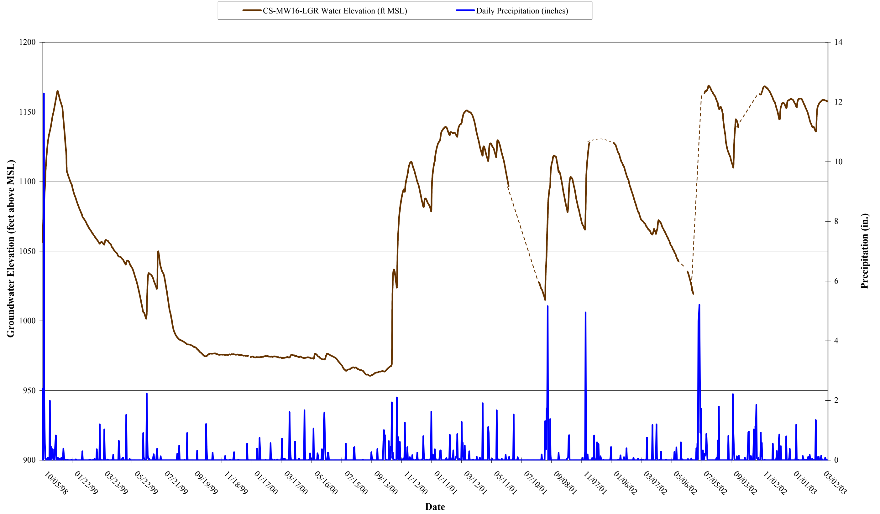
Figure 3-1, Well CS-MW16-LGR (formerly CS-16) Groundwater Elevation and Precipitation Data
