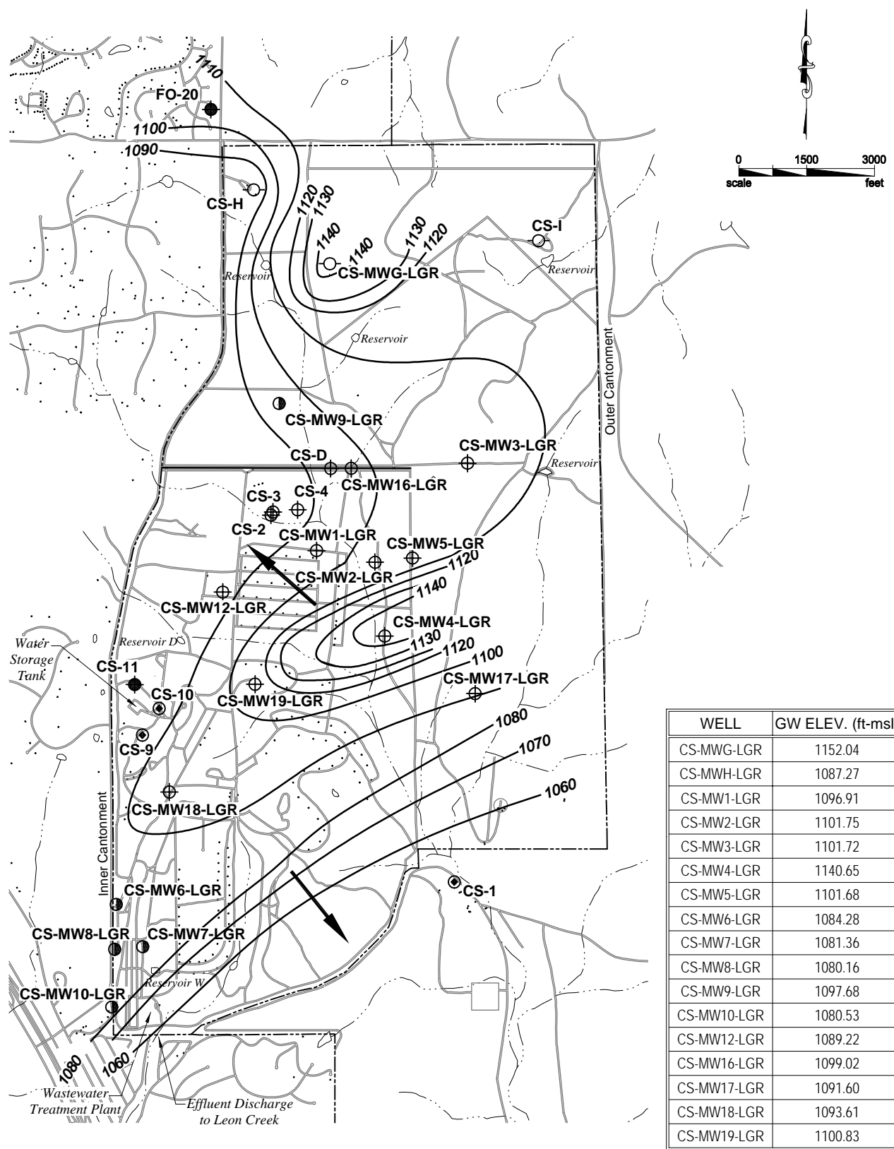
Figure 2.1 Lower Glen Rose Potentiometric Surface Map June 2003 Camp Stanley Storage Activity
