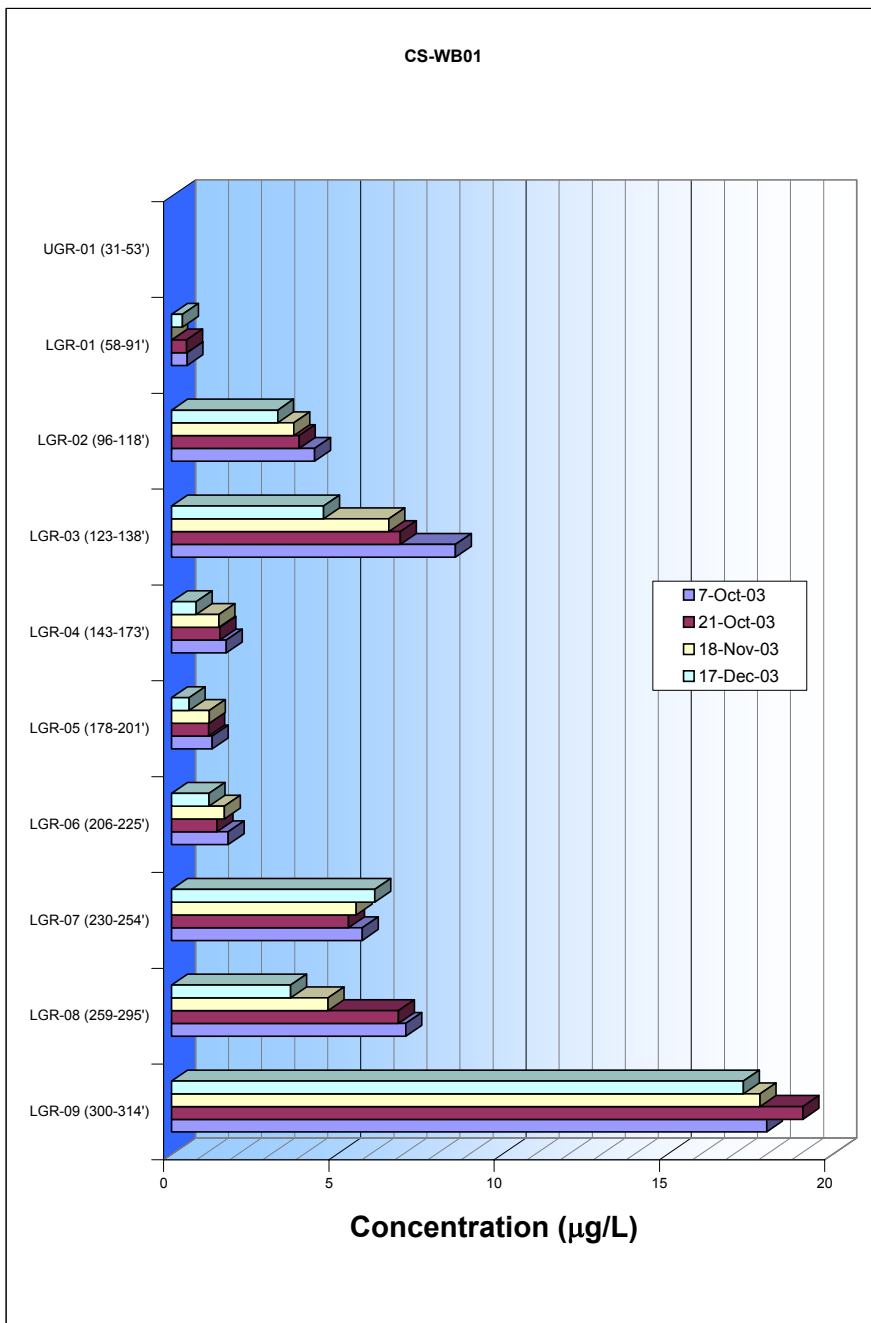
Figure 4-1, October to December 2003 TCE Results Westbay® Wells
