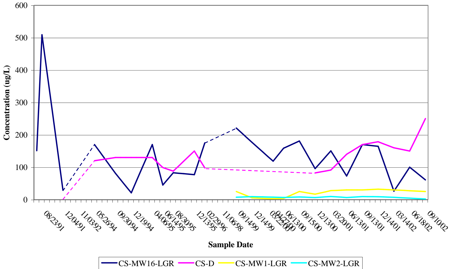
Figure 5-2 Concentrations of Trichloroethene in Selected Wells MCL = 5 ug/L
