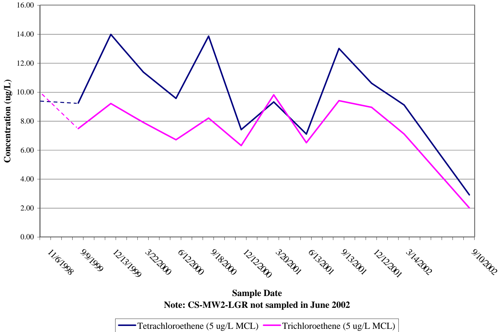
Figure 4-6, Well CS-MW2-LGR PCE and TCE Concentrations since 1998
