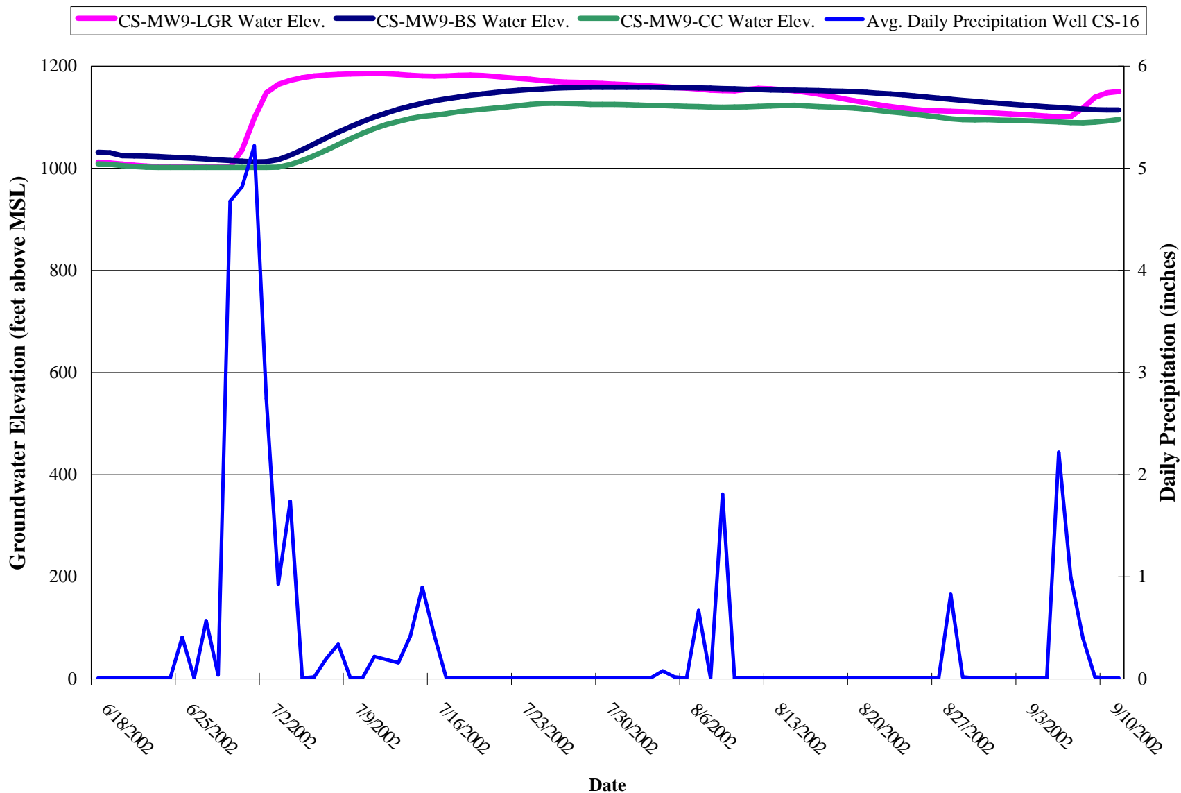
Figure 3-3, Well CS-MW9 Cluster Groundwater Elevation and Precipitation Data
