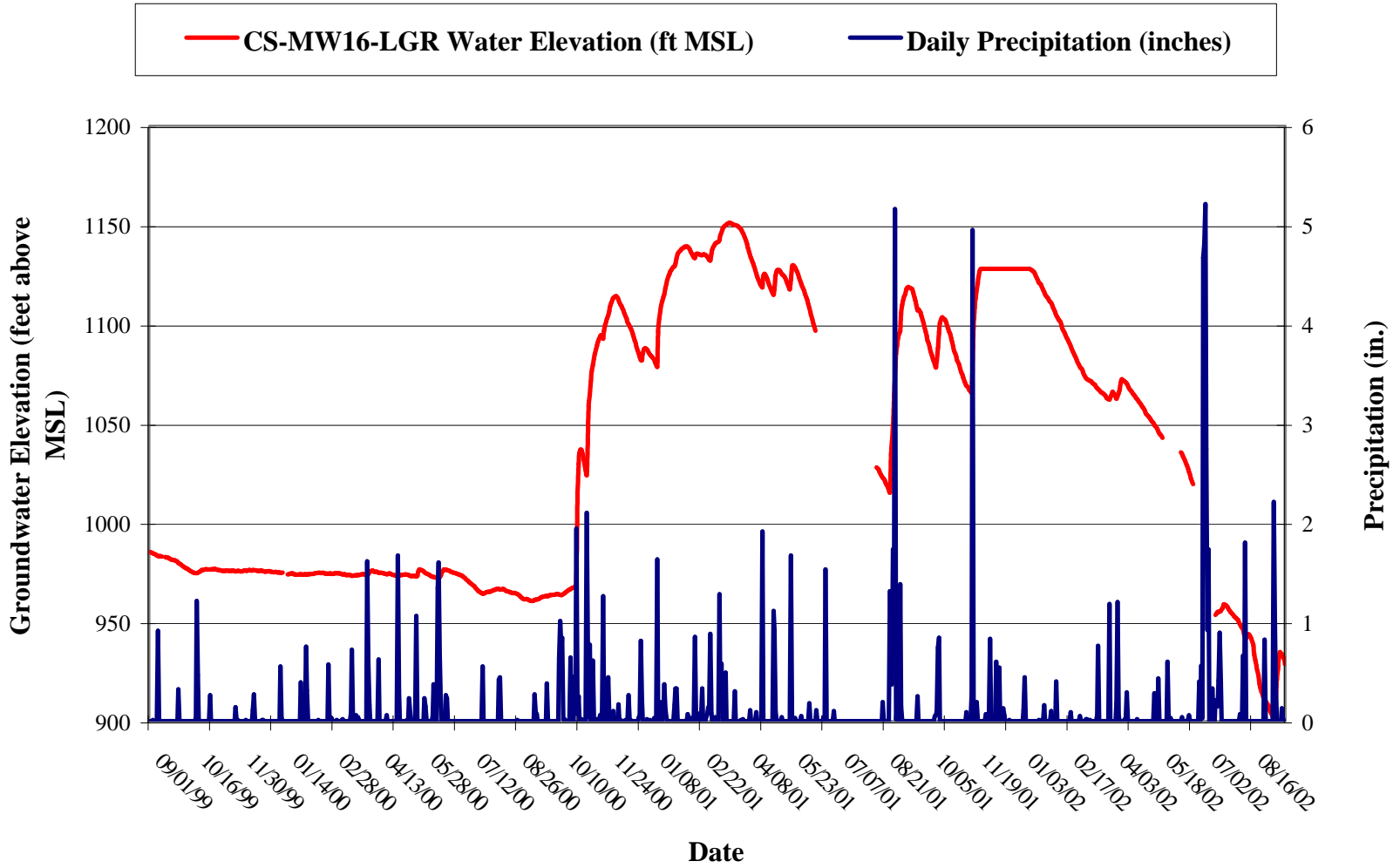
Figure 3-1, Well CS-MW16-LGR Groundwater Elevation and Precipitation Data
