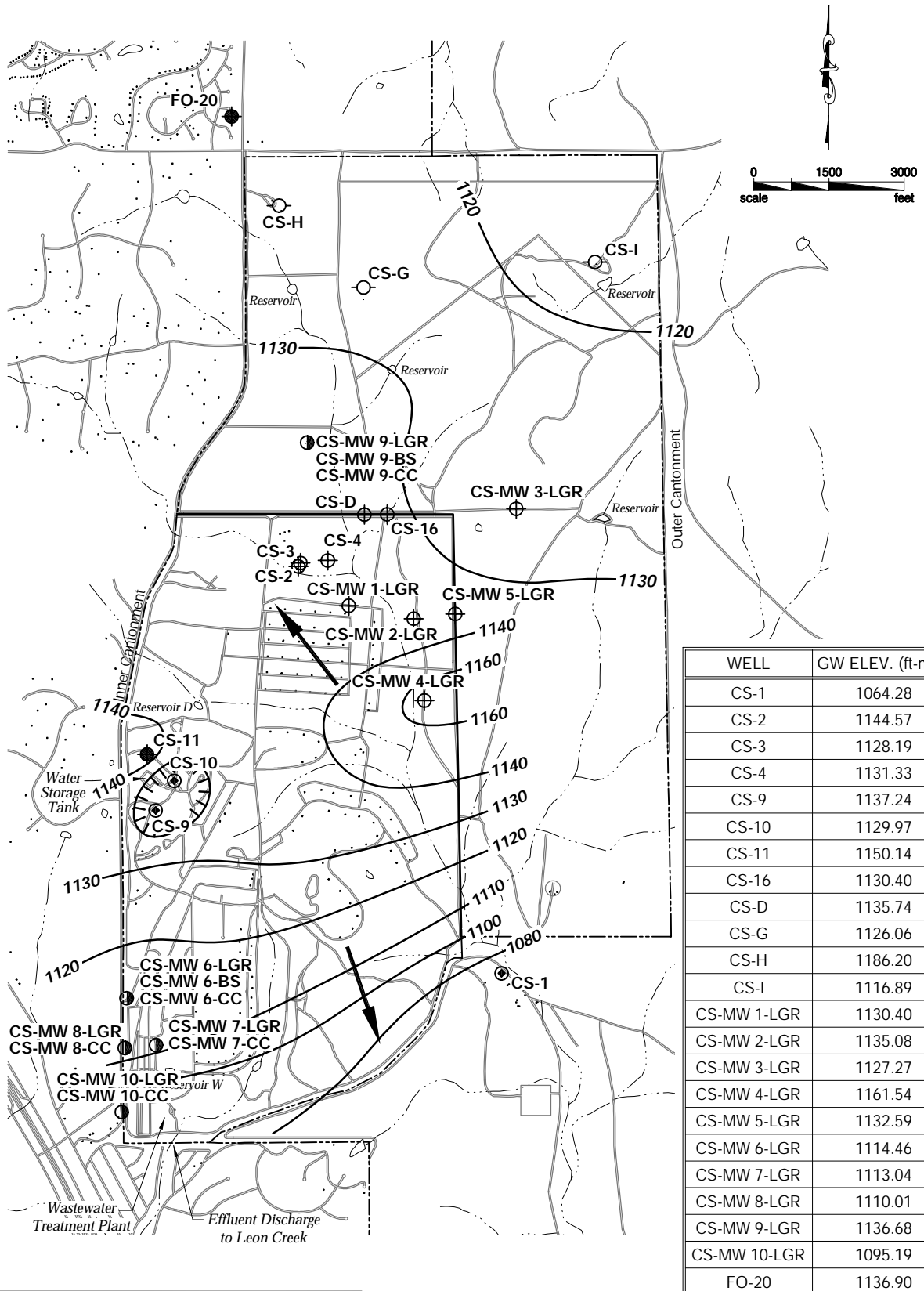
Figure 2-1 Potentiometric Surface Map September, 2002 Camp Stanley Storage Activity
