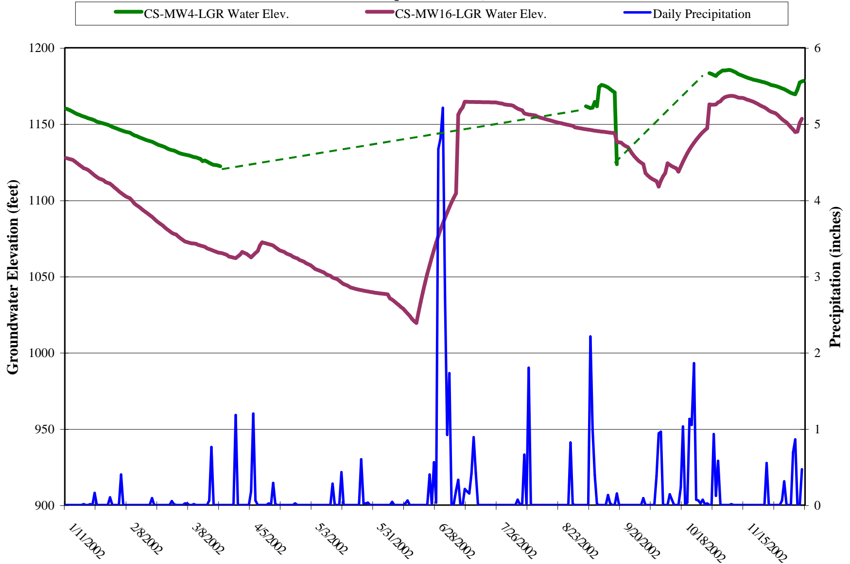
Figure 3-3, Wells CS-MW16-LGR & CS-MW4-LGR Groundwater Elevations and Precipitation Data, December 2002
