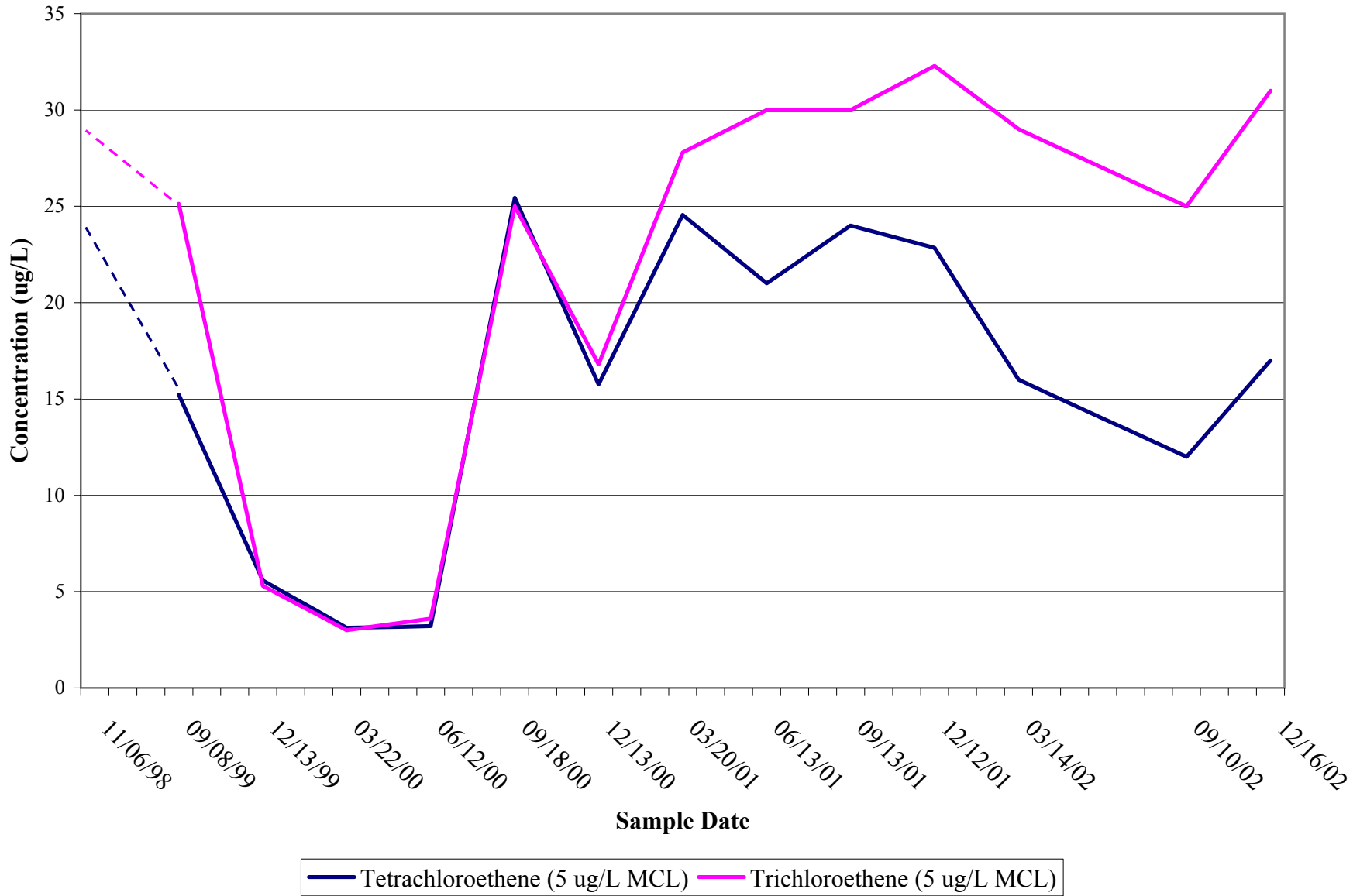
Figure 4-5, Well CS-MW1-LGR PCE and TCE Concentrations since 1998
