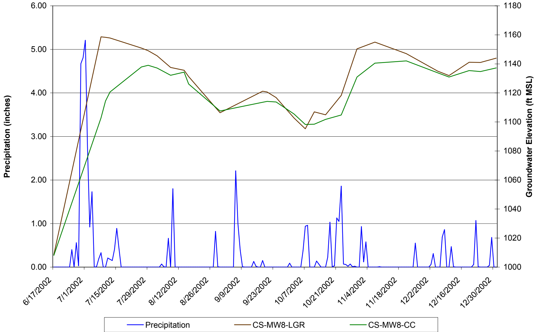
Figure 2-6, Groundwater Elevations for Wells CS-MW8-LGR/CC
