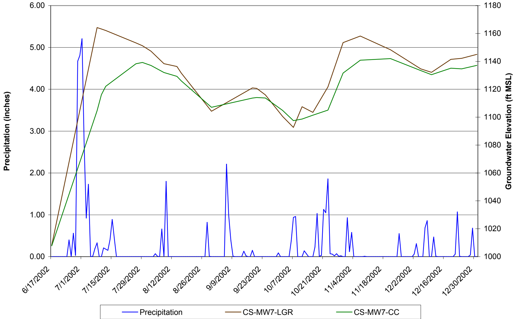
Figure 2-5, Groundwater Elevations for Wells CS-MW7-LGR/CC
