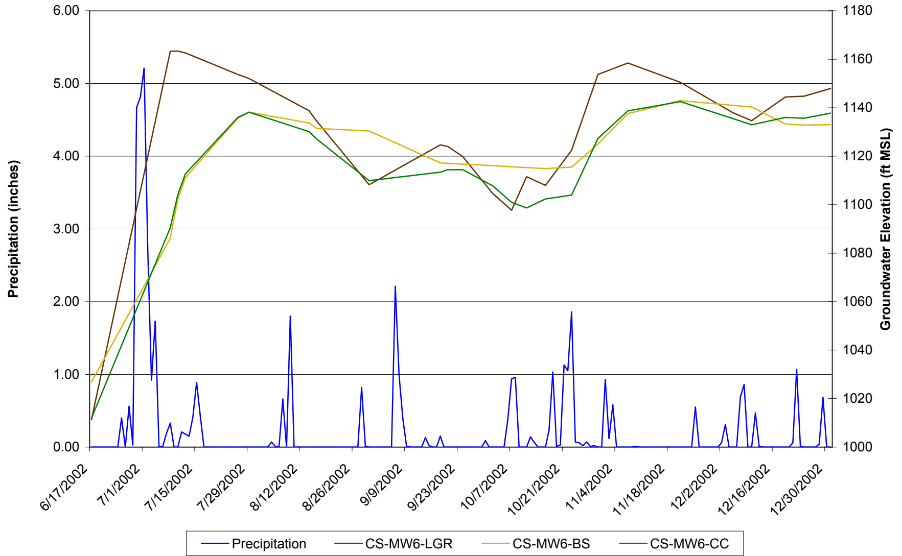
Figure 2-4, Groundwater Elevations for Wells CS-MW6-LGR/BS/CC
