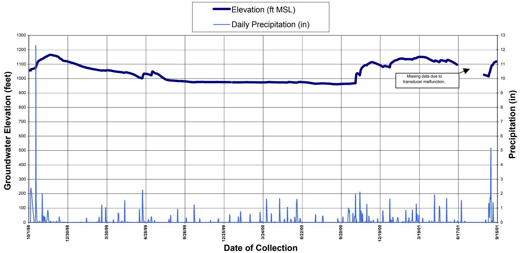
Figure 3 Well CS-16 Groundwater Elevation and Precipitation Data Camp Stanley Storage Activity, Texas
