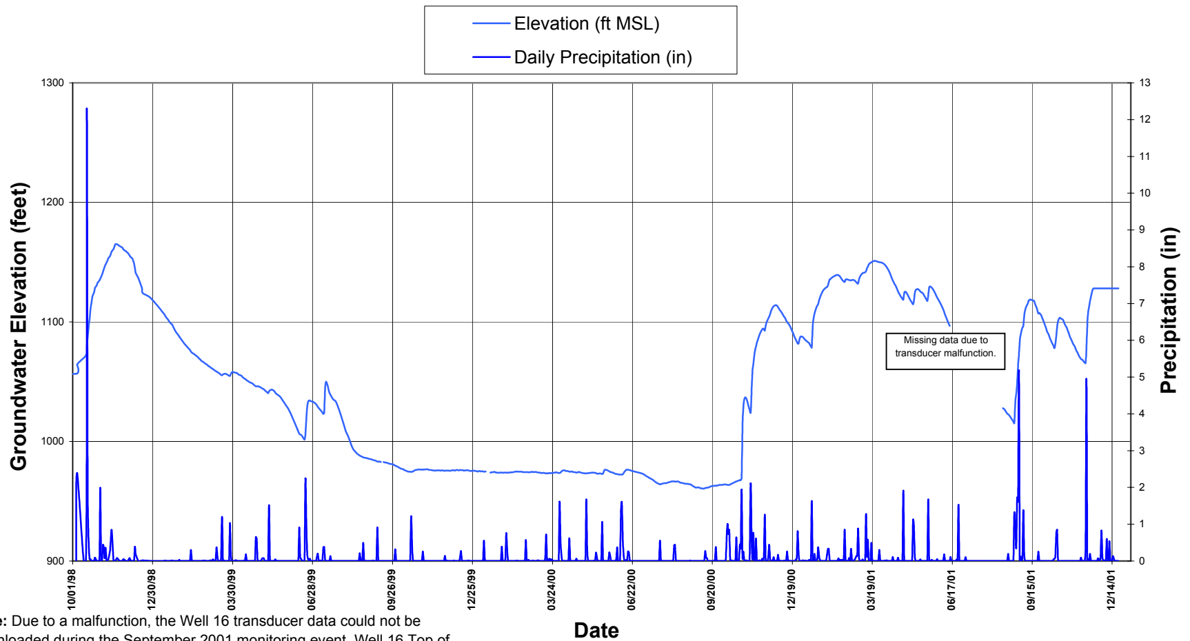
Figure 3-1 Well CS-16 Groundwater Elevation and Precipitation Data Camp Stanley Storage Activity, Texas
