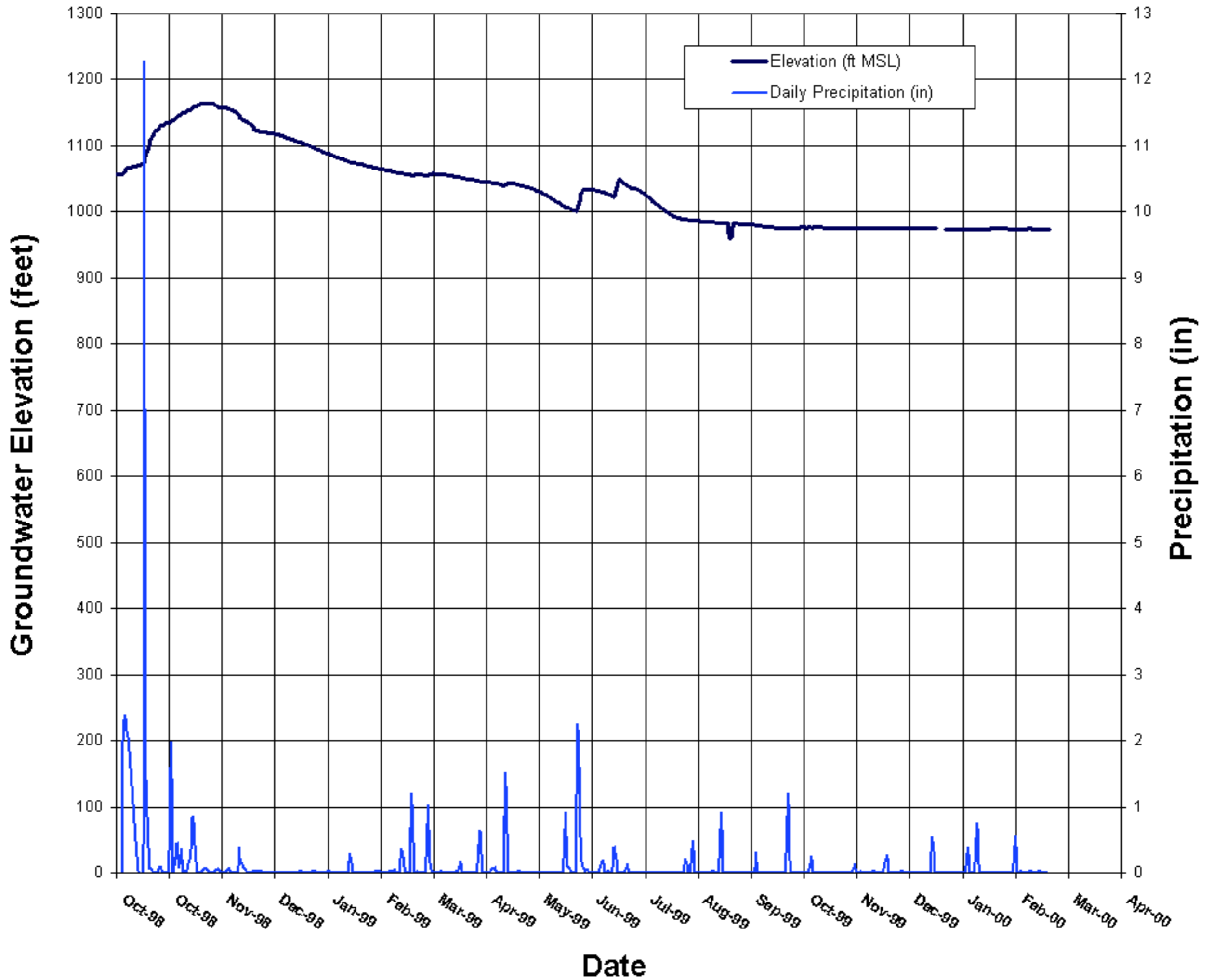
Figure 8 Well 16 Groundwater Elevation and Precipitation Data Camp Stanley Storage Activity, Texas
