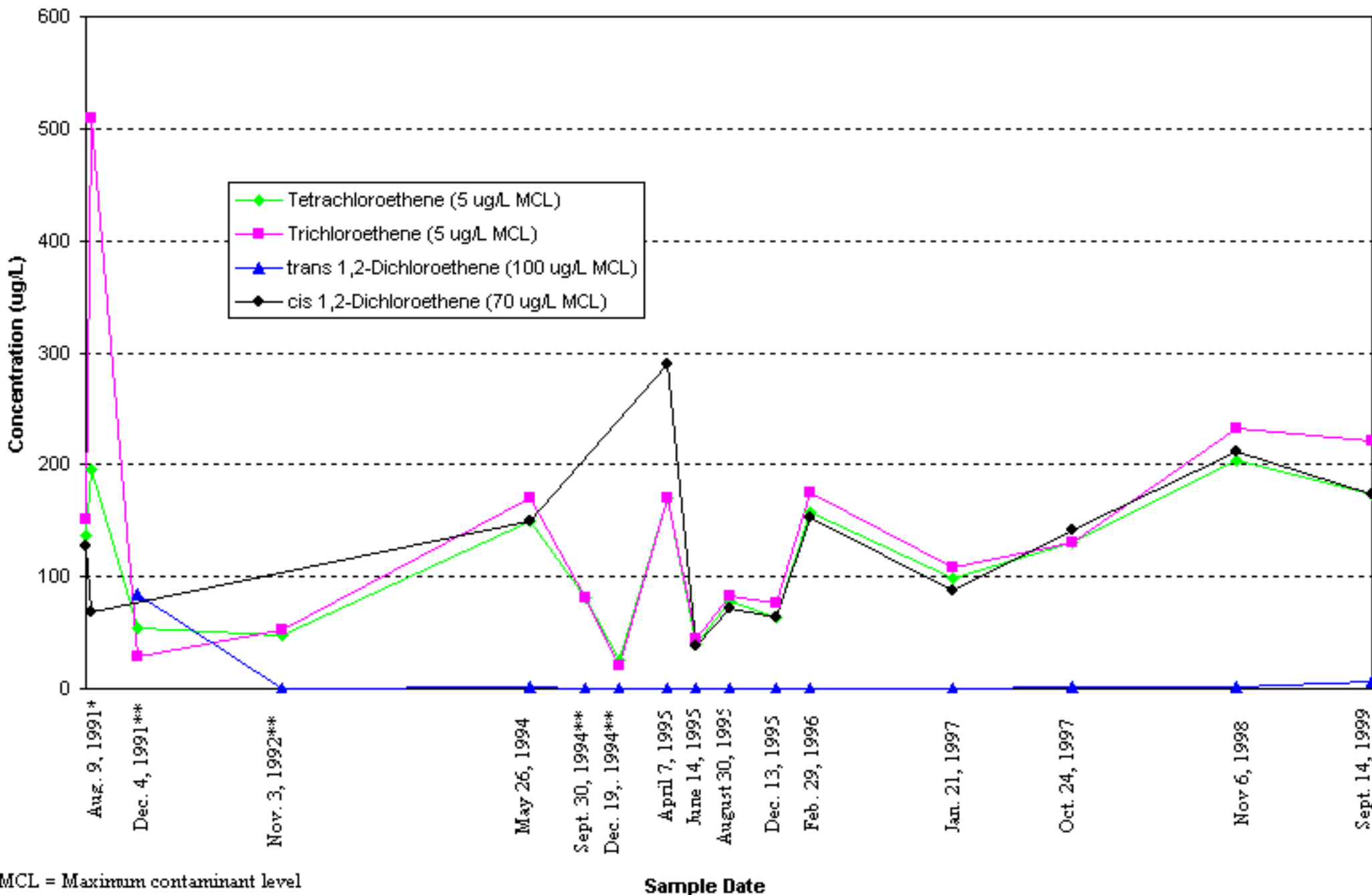
Figure 7 VOC Concentrations Over Time for Well 16, CSSA
