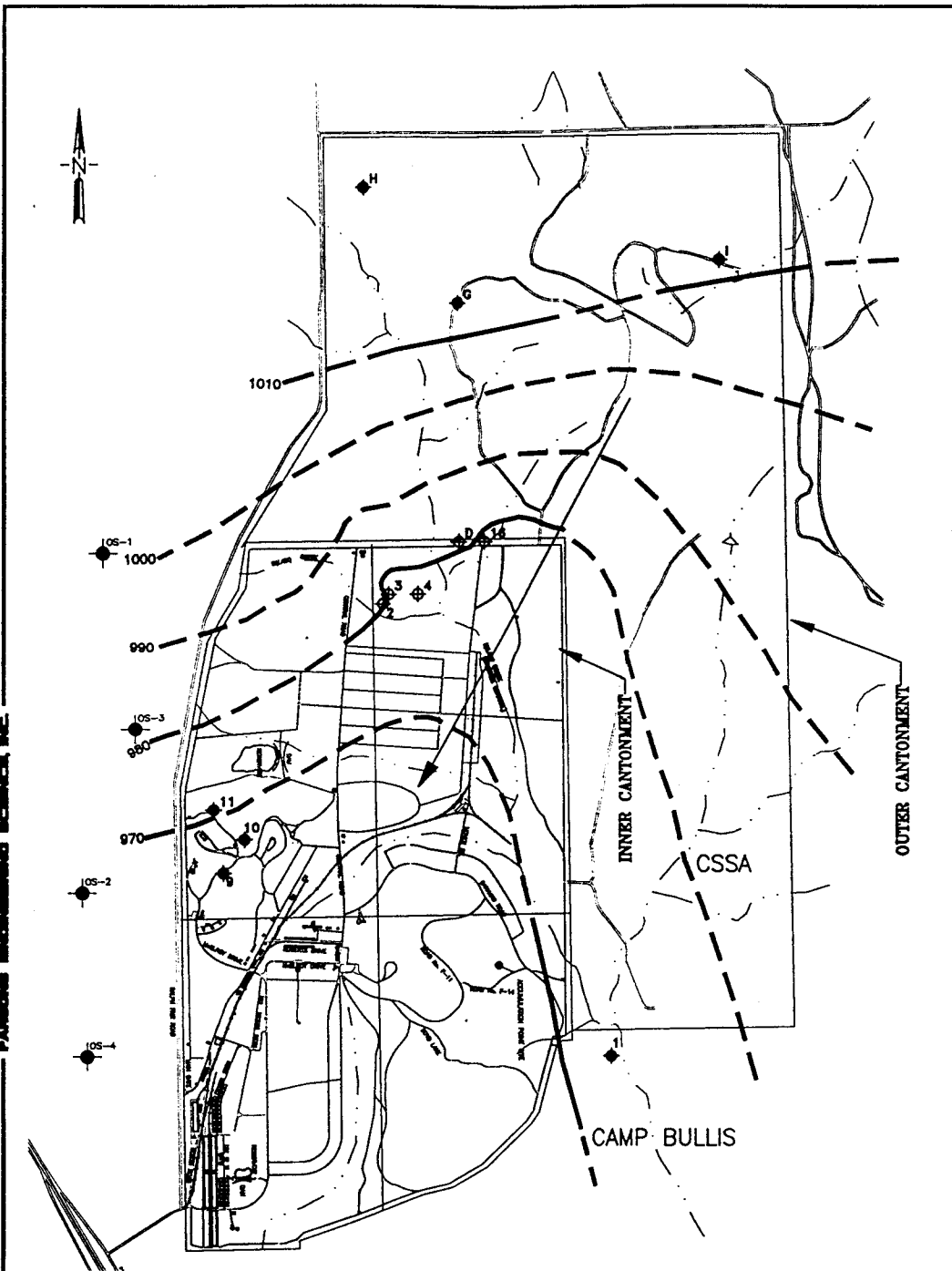
FIGURE 1 GROUNDWATER POTENTIOMETRIC MAP WITHOUT AIRLINE MEASUREMENTS CAMP STANLEY DECEMBER 1995 CSSA GROUNDWATER EVALUATION
