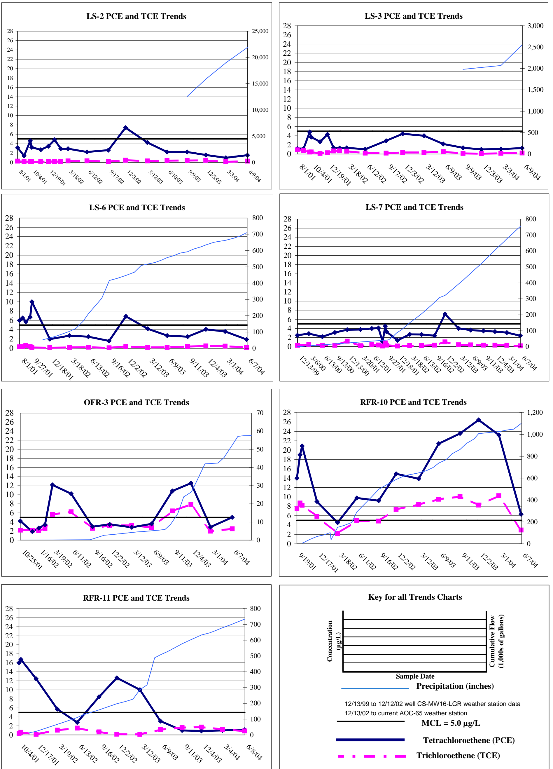
Figure 3.2, PCE and TCE Concentration Trends
