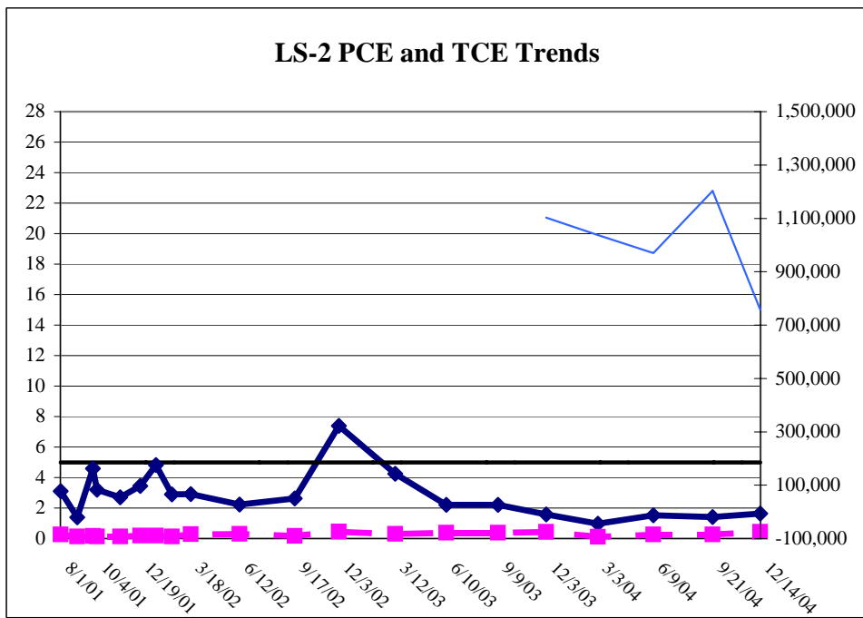
Figure 3.2, PCE and TCE Concentration Trends and Monthly Flow
