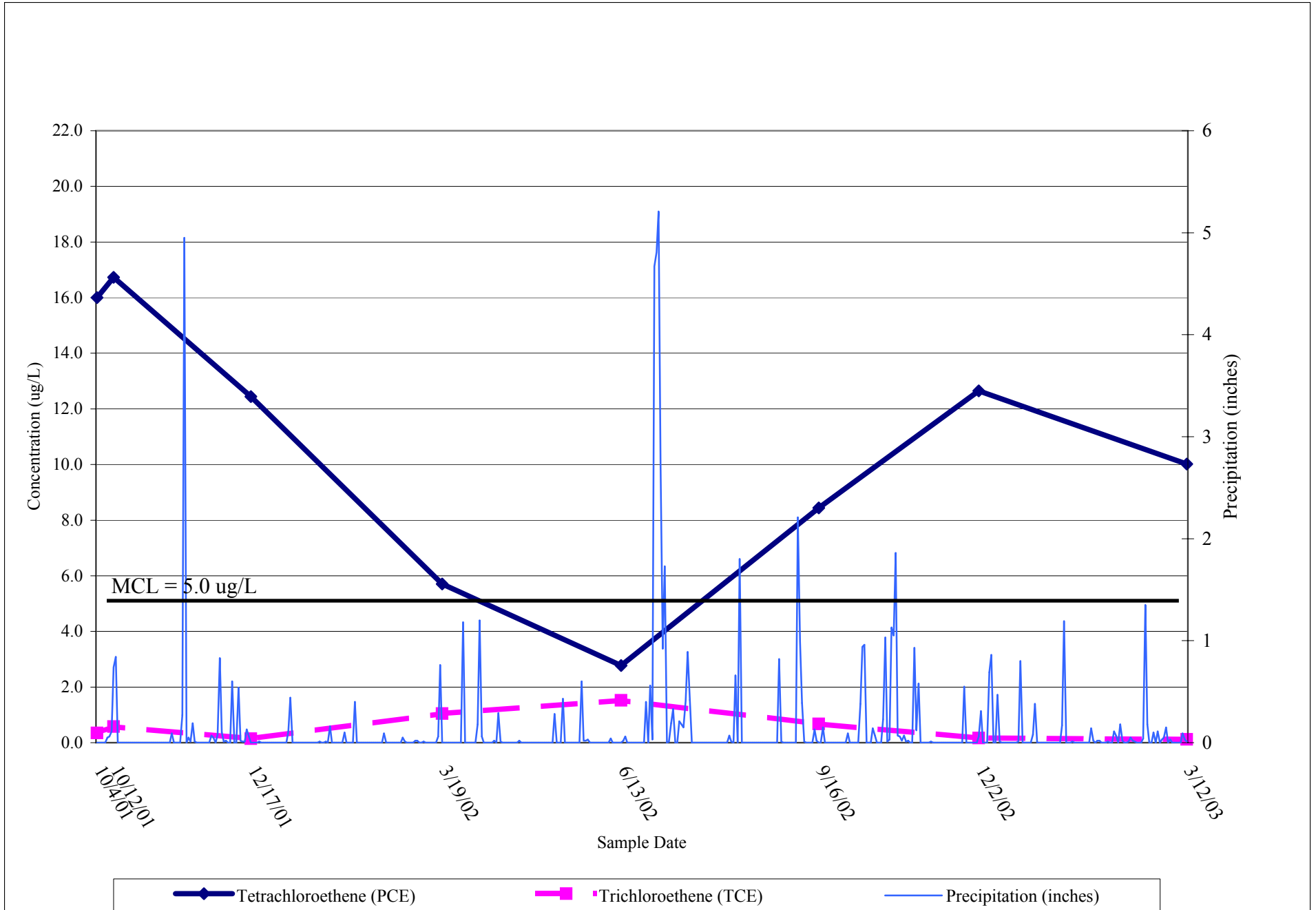
Figure 3.7, RFR-11 TCE and PCE Trends
