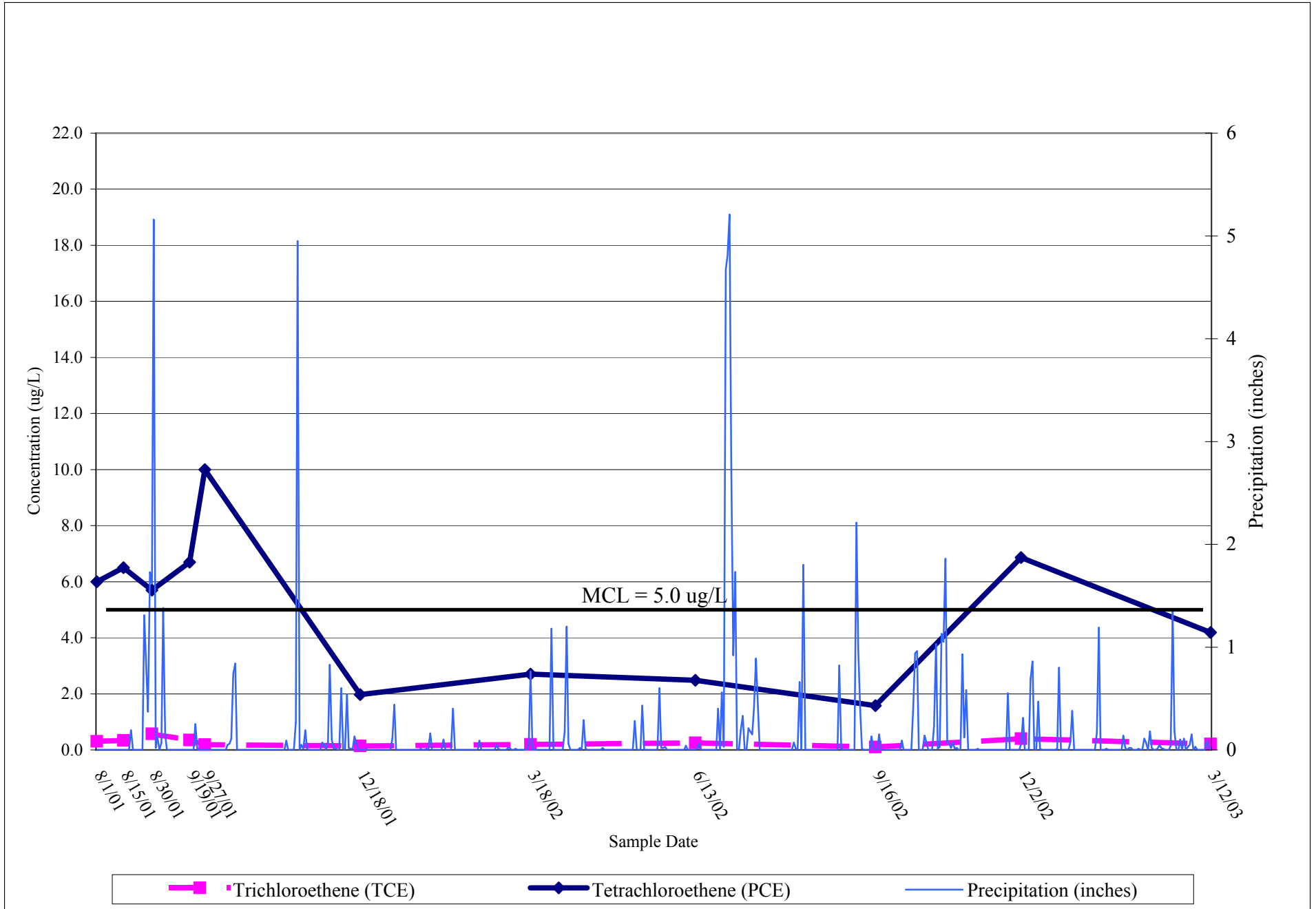
Figure 3.3, LS-6 PCE and TCE Trends
