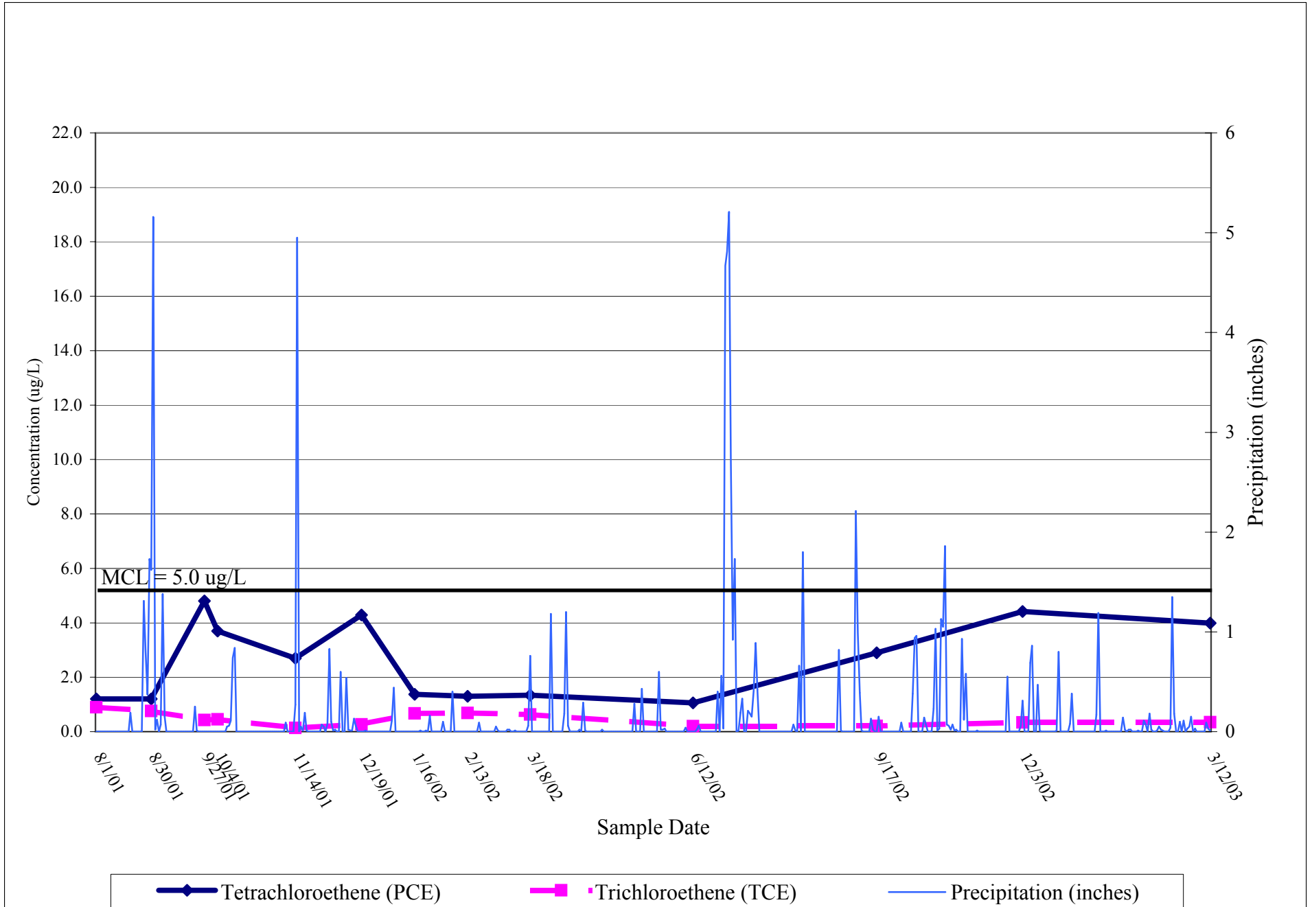
Figure 3.2, LS-3 PCE and TCE Trends
