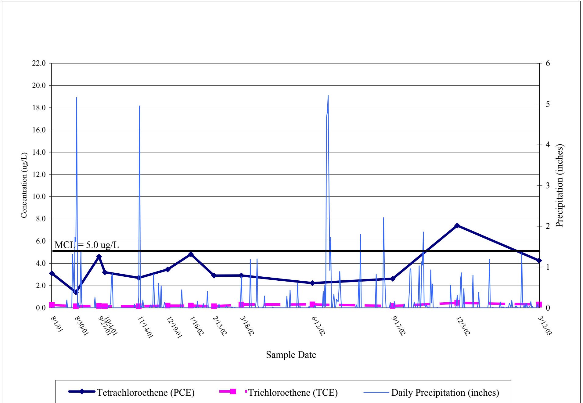
Figure 3.1, LS-2 PCE and TCE Trends vs. Precipitation
