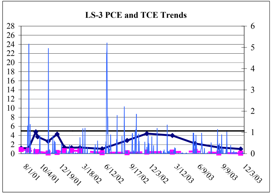
Figure 3.1, PCE and TCE Concentration Trends
