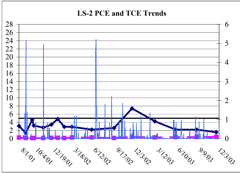
Figure 3.1, PCE and TCE Concentration Trends
