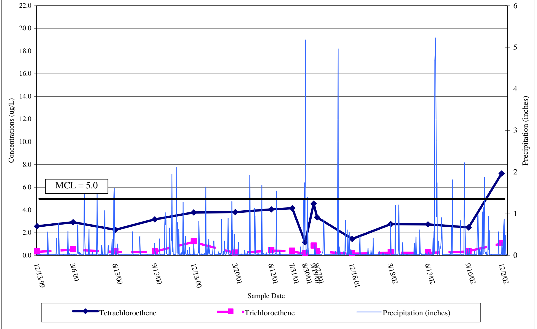
Figure 3.4, LS-7 PCE and TCE Trends
