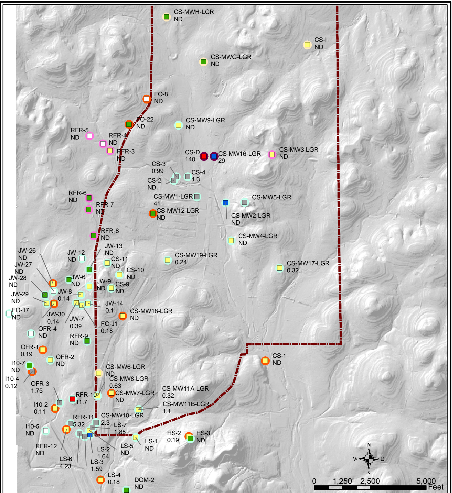
FIGURE 5.5 TEMPORAL TREND RESULTS FOR PCE LGR ZONE WELLS LONG TERM MONITORING OPTIMIZATION CAMP STANLEY STORAGE AREA, TEXAS PARSONS
