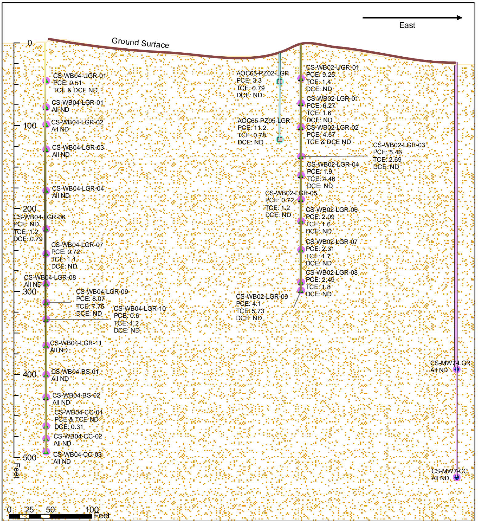
FIGURE 3.7 DECEMBER 2004 OR MOST RECENT COC CONCENTRATIONS WEST-EAST CROSS SECTION AOC65 AREA
