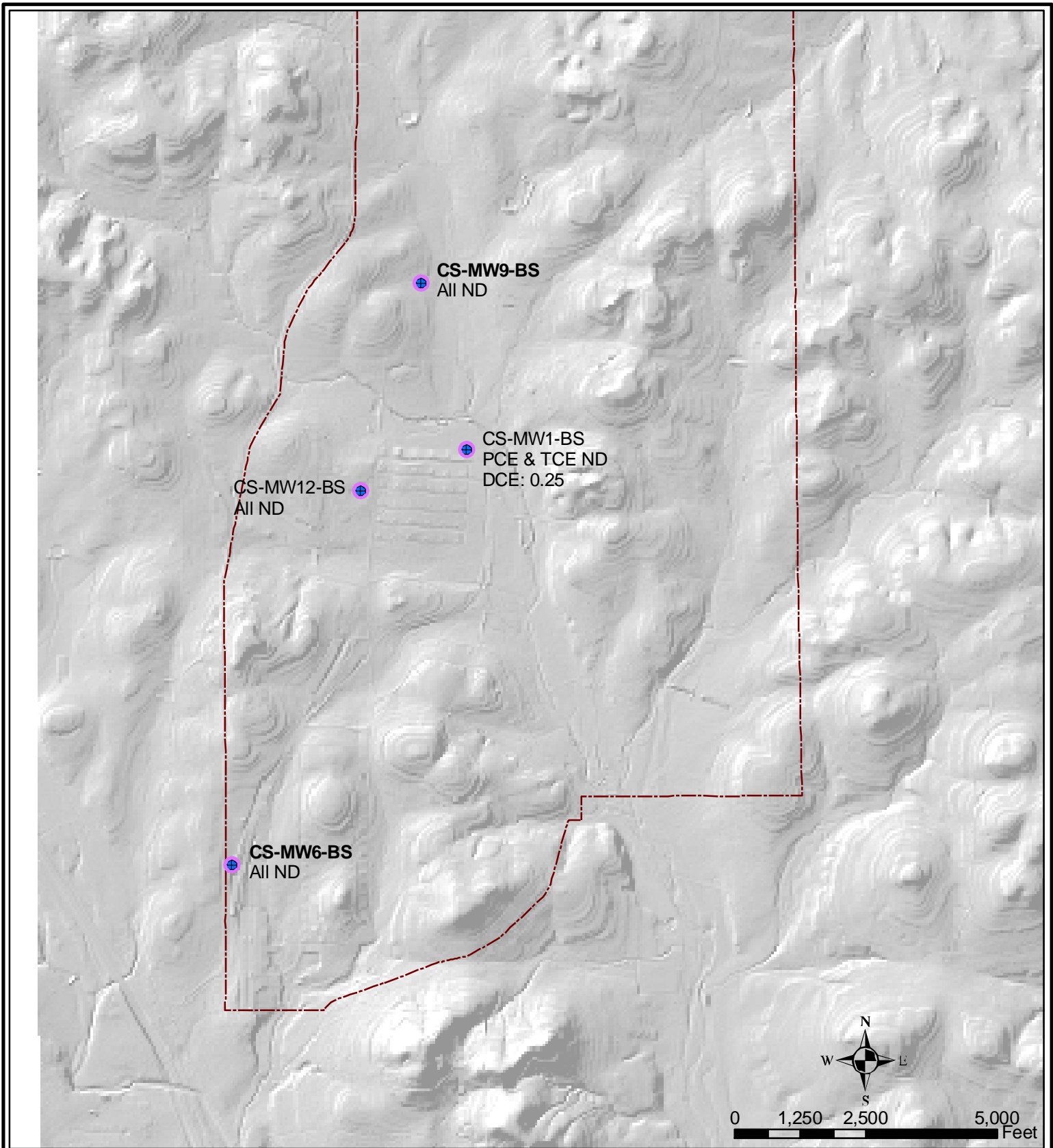
FIGURE 3.4 DECEMBER 2004 OR MOST RECENT SAMPLING EVENT COC CONCENTRATIONS BS ZONE WELLS LONG TERM MONITORING OPTIMIZATION CAMP STANLEY STORAGE AREA, TEXAS PARSONS
