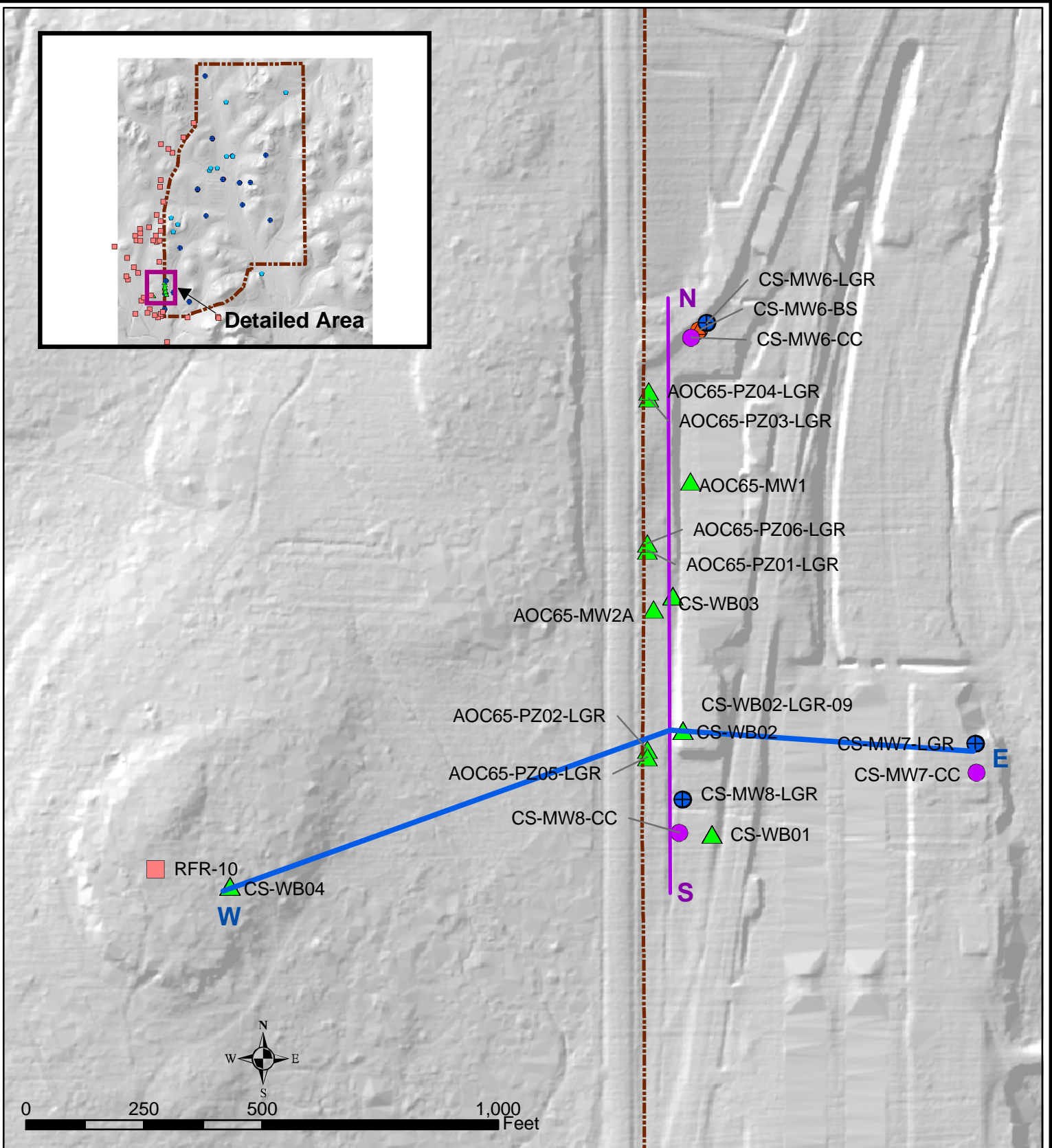
FIGURE 3.2 GROUNDWATER MONITORING WELLS & CROSS SECTIONS AOC65 AREA LONG TERM MONITORING OPTIMIZATION CAMP STANLEY STORAGE AREA, TEXAS PARSONS
