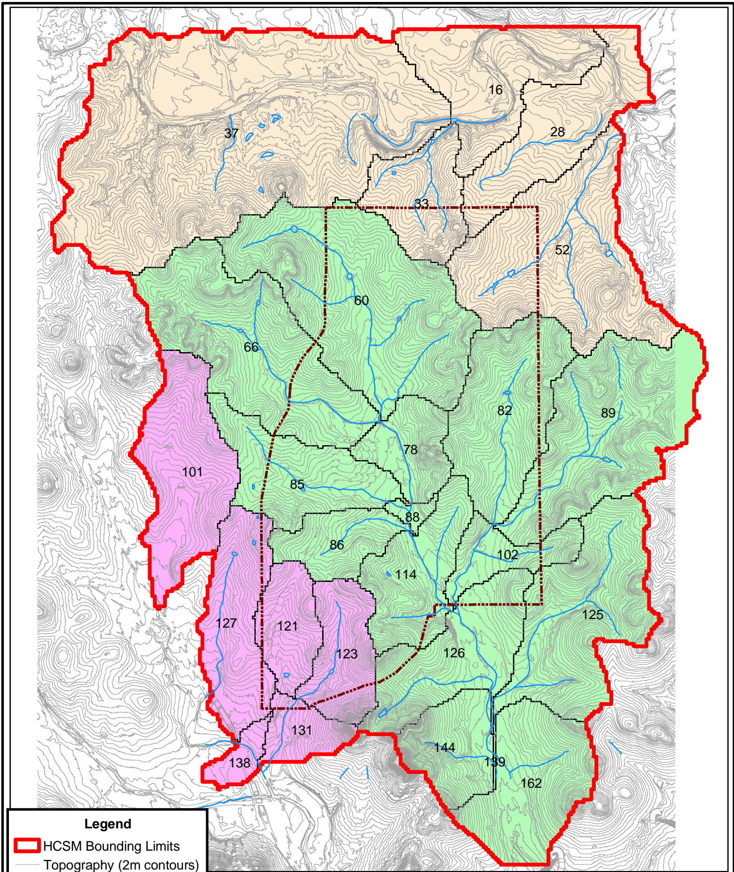
Figure 4.31 Model Area Watershed Subunits based on USGS Digital Elevation Model (2001) PARSONS
