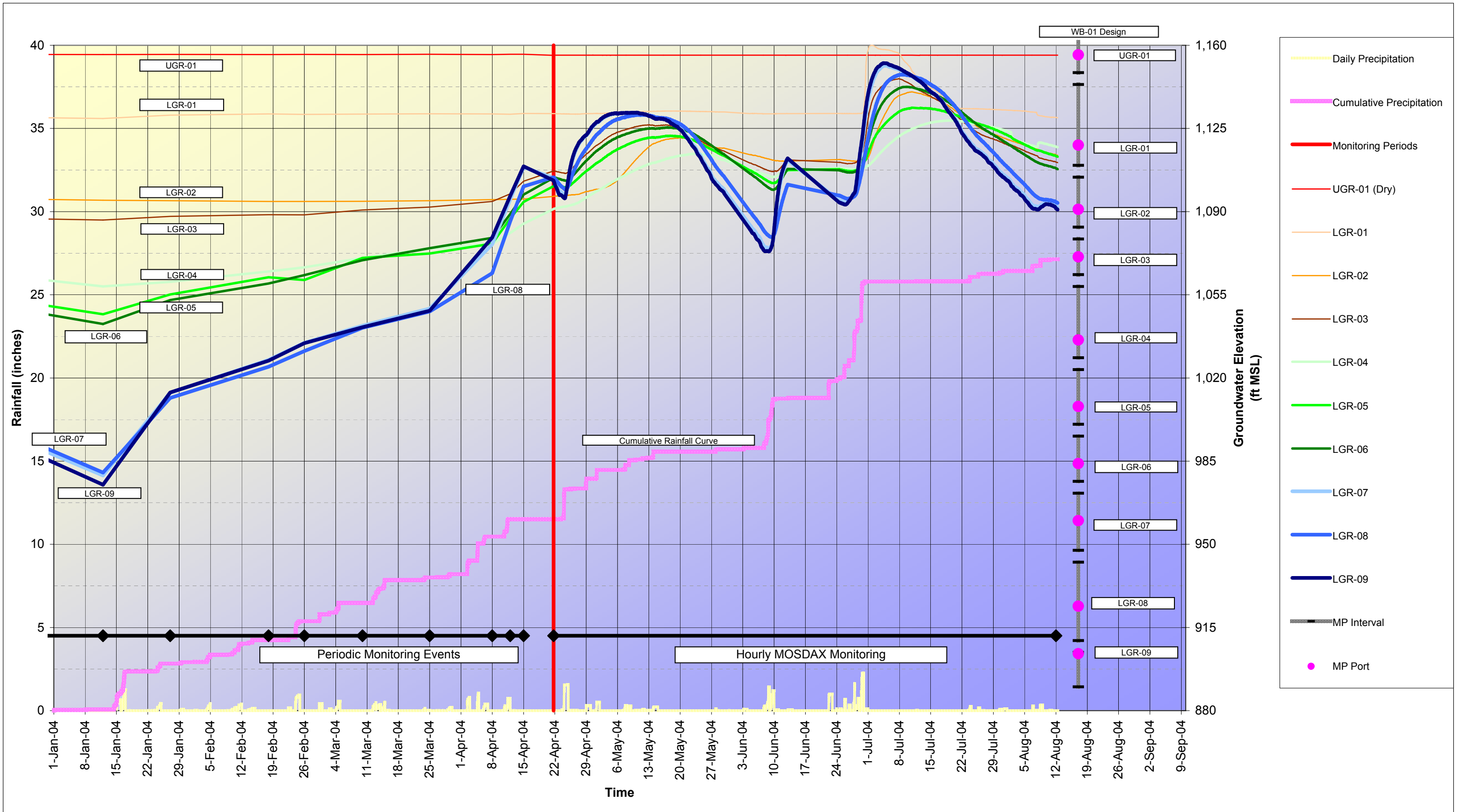
Figure 4.28 CS-WB01 Hydraulic Profiling Data January - August 2004
