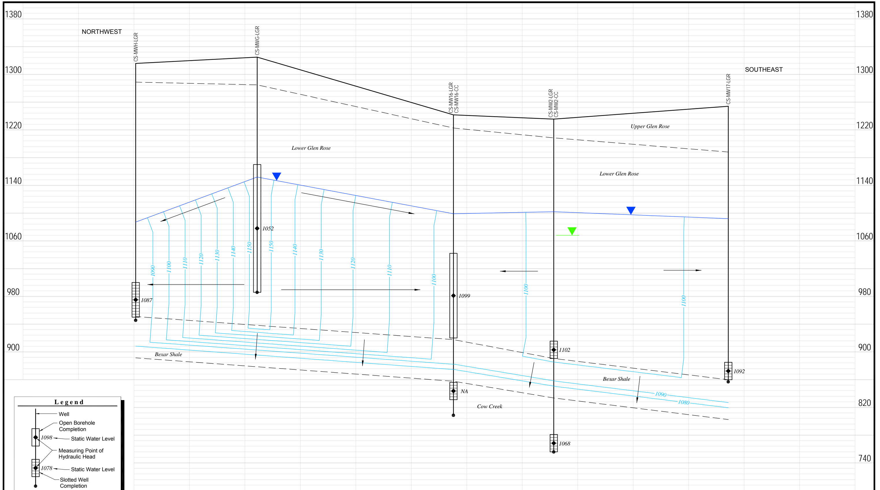
Figure 4.27 Flow net of Potential Hydraulic Head, June 2003 (Northwest to Southeast Profile) Camp Stanley Storage Activity, Texas PARSONS
