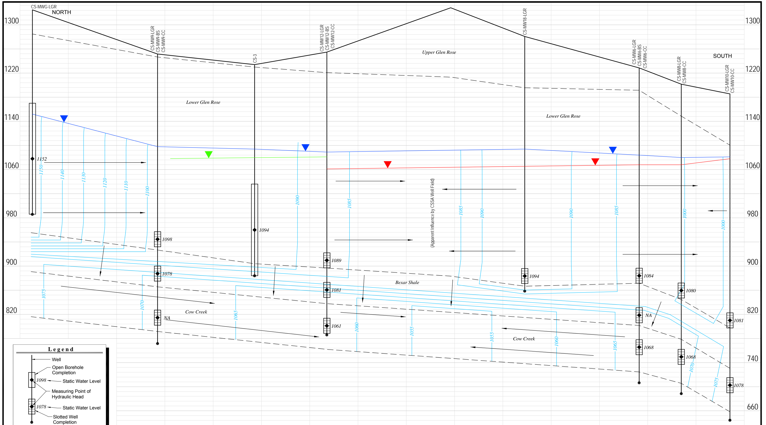
Figure 4.26 Flow net of Potential Hydraulic Head, June 2003 (North to South Profile) Camp Stanley Storage Activity, Texas PARSONS
