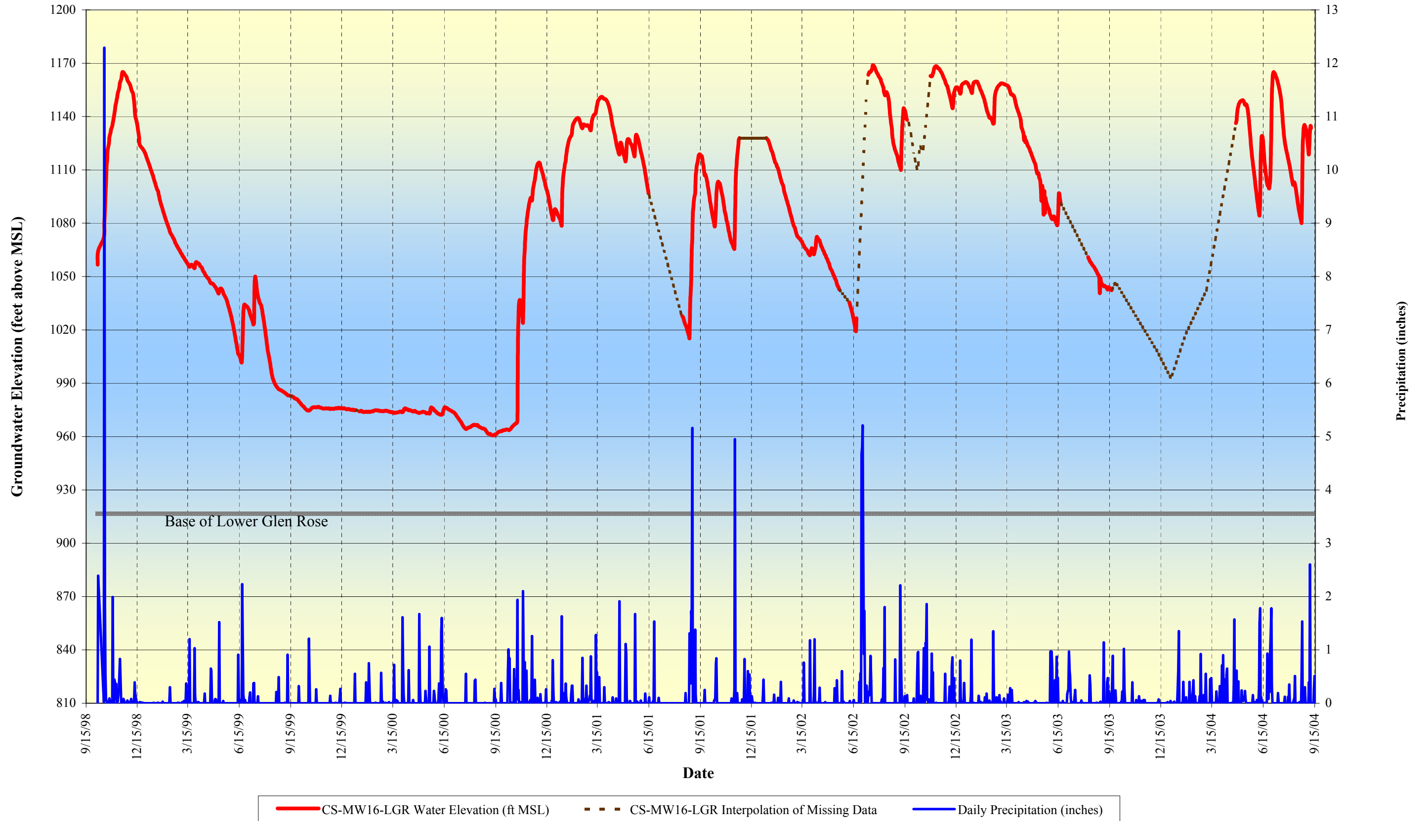
Figure 4.23 Hydrograph of Well CS-MW16-LGR and Precipitation Data
