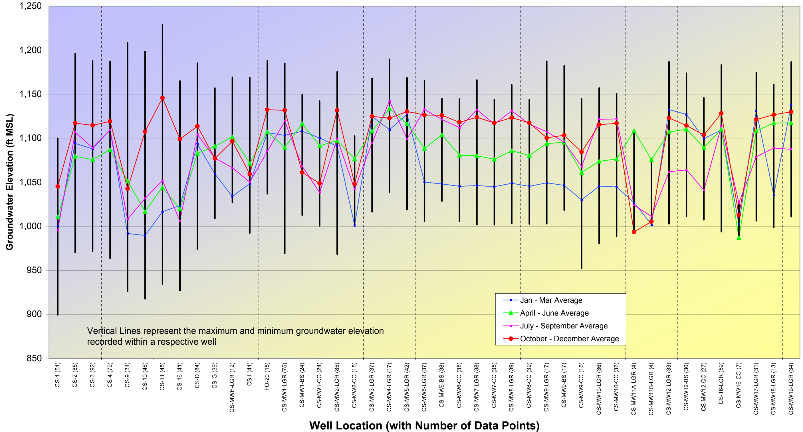
Figure 4.22 Seasonal Groundwater Fluctuations in Selected Wells 1992-2004 Camp Stanley Storage Activity - Boerne, TX
